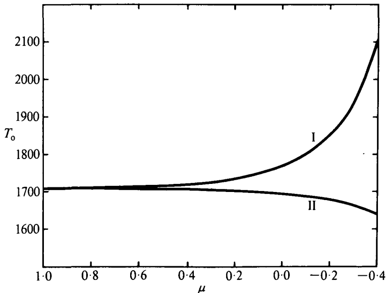
FIG. 3. The zeroth-order value T_0(\delta) of the critical Taylor number is plotted versus \mu on curve I. The second curve II is the corresponding plot for infinite coaxial cylinders.
