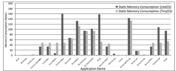
d) Static Memory Consumption Comparison
