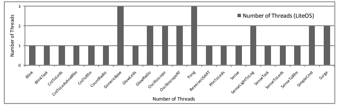
a) Number of Threads for LiteOS Applications
