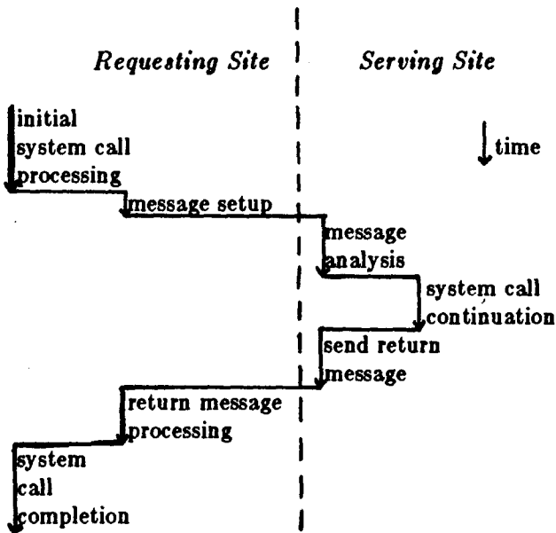
Figure 1: Processing a System Call Requiring Foreign Service
