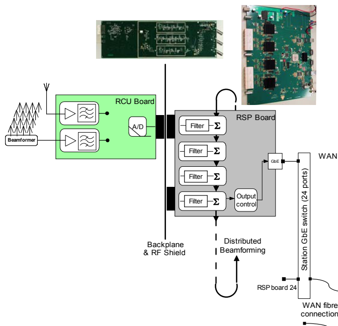
Figure 1: The main station architecture, showing the antennas, the receiver (RCU board, green), the digital signal processing (RSP board, grey) and the wide-area network (WAN) interface.
