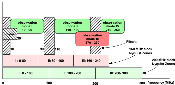
Figure 2: The available modes in the LOFAR receiver, selecting one of three Nyquist zones for the two available clock rates.
