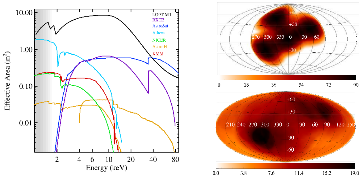
Figure 9. Left: The effective area of LOFT/LAD as compared to the largest past, on-going and approved missions. The shaded area below 2 keV indicates the fact that the LAD will outperform its science requirement of 2 keV low energy threshold, by extending its sensitivity down to \leq 1.5 keV, beneficial to the study of complex absorption structures. Right: Map in Galactic coordinates of the active detector area for a sample observation performed in the direction of the Galactic centre (top) and 1yr Exposure map in Galactic coordinates for positions covered by at least 10 \text{ cm}^2 per observation. Map scale is given in Ms.
