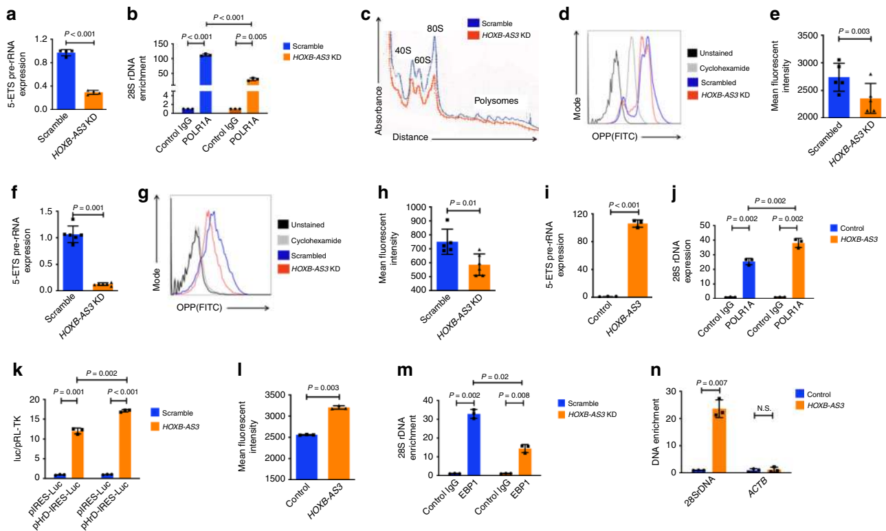
Fig. 5 HOXB-AS3 regulates rRNA transcription via guiding the EBP1 protein to the rDNA locus. a Relative pre-rRNA expression in OCI-AML3 cells treated with scramble or anti-HOXB-AS3 gampers. b Occupancy of ribosomal DNA promoter repeat sequence (28S rDNA) by POLR1A in scramble versus HOXB-AS3 KD OCI-AML3 cells. c Sucrose gradient-based isolation and quantification (via ultraviolet radiation absorbance) of ribosomes and polysomes in scramble versus HOXB-AS3 KD OCI-AML3 cells. d Effect of HOXB-AS3 depletion on de novo protein synthesis in OCI-AML3 cells, The flow cytometry graph from one representative experiment is shown. e Comparison of the mean fluorescence intensity of the Alexa Fluor 488-positive OCI-AML3 cells treated with scramble versus HOXB-AS3 KD, in de novo protein synthesis assays. Results of four independent experiments are shown. f Relative 5-ETS pre-rRNA expression in human AML patient blasts treated in vivo with scramble versus anti-HOXB-AS3 gampers. Results of three scramble and four HOXB-AS3 KD-treated mice are depicted in aggregate. g, h Effect of HOXB-AS3 KD on de novo protein synthesis in in vivo treated human AML blasts. i Relative pre-rRNA expression in K-562 cells transfected with empty vector (control) or HOXB-AS3 overexpressing vectors. j Occupancy of 28S rDNA by POLR1A in K-562 cells transfected with control or HOXB-AS3 overexpressing vectors. k Relative luciferase-reporter (luc/pRL-TK) activity in K-562 cells transfected with empty control (pIRES-Luc) or rDNA-promoter-containing (pHrD-IRES-Luc) luciferase-reporter vectors, and control or HOXB-AS3 overexpressing vectors. l Comparison of the mean fluorescence intensity of the Alexa Fluor 488-positive K-562 cells, transfected with control or HOXB-AS3 overexpressing vectors in de novo protein synthesis assays. Results of three independent experiments are shown. m Occupancy of 28S rDNA by EBP1 in scramble versus HOXB-AS3 KD OCI-AML3 cells. n Enrichment of 28S rDNA or the ACTB promoter region in RAP-DNA-based isolation of chromatin with control or HOXB-AS3 hybridizing biotinylated probes. P values were calculated using paired two-sided t -tests. In the figures, heights of boxplots indicate mean values with standard deviation. Error bars indicate highest and lowest values in each population. Source data are provided as a Source Data file.
