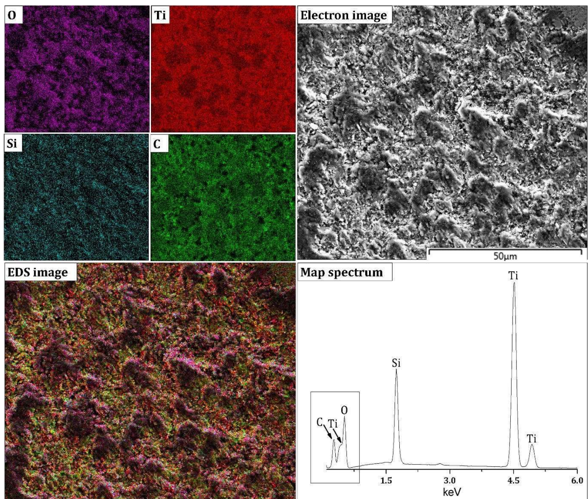
Fig. 7. EDX elemental distribution map and spectrum inside the wear track of the Maxthal 312/ \text{Al}_2\text{O}_3 worn section from wear conditions 100 rpm / 60 min.
