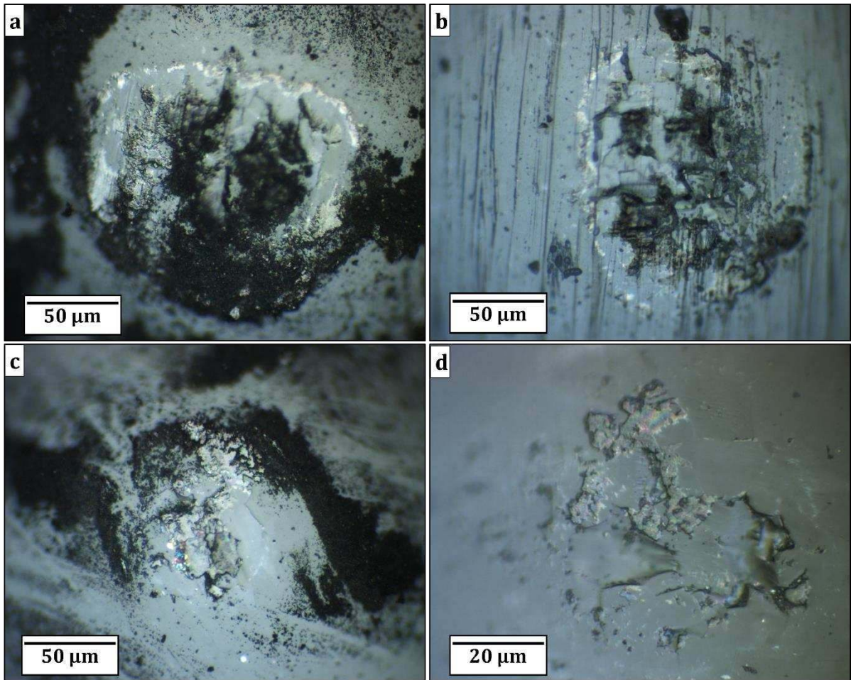
Fig. 12. Optical images of the Al 2 O 3 ball surface after unlubricated sliding against the Maxthal 312 disc ((a) before cleaning and (b) after cleaning) and Maxthal 312-TiC disc ((c) before cleaning and (d) after cleaning) discs for the contact condition 100 rpm for 60 min.
