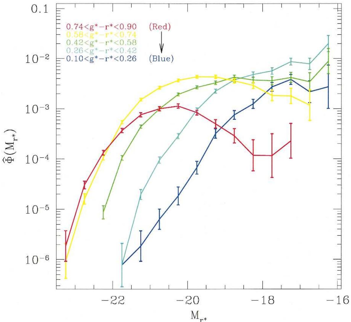
FIG. 14.—Same as Fig. 11, only now showing the luminosity function in bins of intrinsic g^*-r^* color, in units of galaxies per h^{-3} \text{ Mpc}^3 per unit magnitude. As labeled, the curves are colored blue, cyan, green, yellow, and red from bluest to redder. The intrinsic color is determined using the observed color, the measured redshift, and the results of Fukugita et al. (1995). Errors in the calibration used for this data probably broaden this distribution slightly, by about 0.05 mag.
