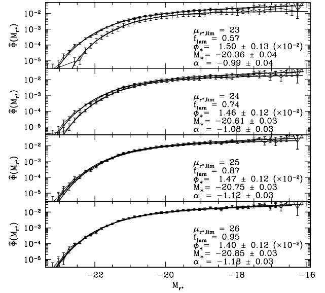
FIG. 21.—Fitted r^* luminosity function for Petrosian magnitudes ( top curve in each panel ; same as Fig. 5) compared with the luminosity function using isophotal magnitudes ( bottom curve in each panel ). Each panel corresponds to a different choice of limiting isophotal surface-brightness \mu_{r^*,\text{lim}} , as labeled. The Schechter function parameters for each choice of isophotal limit are listed in each panel, as well as the fraction f_{\text{lum}} of the total Petrosian luminosity that is detected in each isophotal sample.
