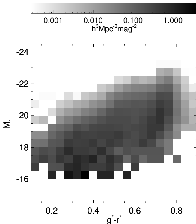
FIG. 13.—Same as Fig. 10, for the joint luminosity-color distribution \hat{\Phi}(M_{r^*}, g^* - r^*) in r^* for SDSS galaxies, now in units of galaxies per h^{-3} \text{Mpc}^3 per unit magnitude per unit color. The intrinsic g^* - r^* colors are inferred using the observed g^* - r^* color, the measured redshift, and the results of Fukugita et al. (1995). The “E/S0” ridge at g^* - r^* \approx 0.75 is apparent, as is the strong correlation between luminosity and color.
