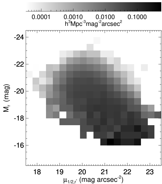
FIG. 10.—Logarithmic gray scale representing \hat{\Phi}(M_{r^*}, \mu_{1/2,r^*}) in r^* for SDSS galaxies, in units of galaxies per h^{-3} \text{ Mpc}^3 per unit magnitude per unit surface brightness, calculated using the method of Efstathiou, Ellis, & Peterson (1988). The translation of the gray scale to these units is given in the bar at the top of the figure. The data sample has an explicit half-light surface brightness cut at \mu_{1/2,r^*} = 23.5 . The strong correlation between surface brightness and luminosity is apparent. It is clear why many of the objects with \mu_{1/2,r^*} > 22.5 are low luminosity, as shown in Fig. 9.
