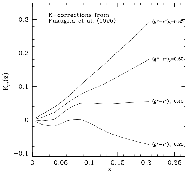
FIG. 4.— K -corrections in the r^* band for galaxies with intrinsic g^* - r^* colors of 0.2, 0.4, 0.6, and 0.8, as labeled. These curves are obtained by linear interpolation between the morphological types used by Fukugita et al. (1995). Similar results are available for the other four bands.
