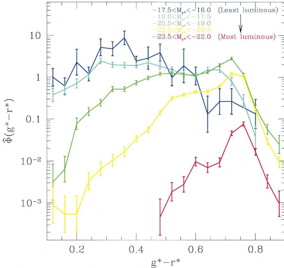
FIG. 15.—Same as Fig. 12, only now showing the distribution of intrinsic g^* - r^* color for several ranges of r^* luminosity, in units of galaxies per h^{-3} \text{Mpc}^3 per unit color. As labeled, the curves are colored blue, cyan, green, yellow, and red from low to high luminosity. As in Fig. 13, the “E/S0” ridge at g^* - r^* \approx 0.75 is apparent for high luminosities, while for low luminosities, the g^* - r^* distribution is nearly flat.
