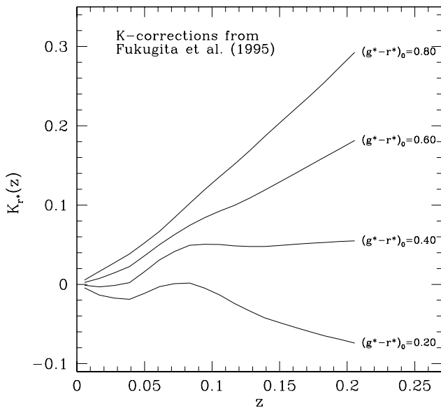
FIG. 4.— K -corrections in the r^* band for galaxies with intrinsic g^*-r^* colors of 0.2, 0.4, 0.6, and 0.8, as labeled. These curves are obtained by linear interpolation between the morphological types used by Fukugita et al. (1995). Similar results are available for the other four bands.
