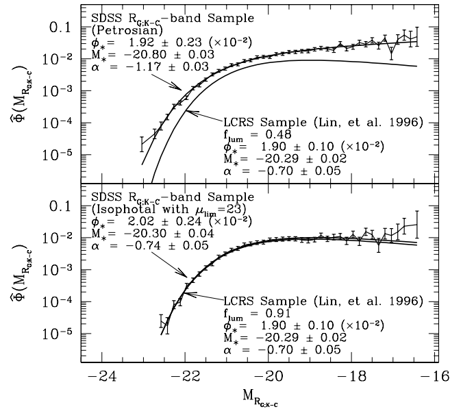
FIG. 22.—R-band luminosity function in the SDSS compared with that in the LCRS calculated by Lin et al. (1996). Top panel : Luminosity function calculated from the SDSS using Petrosian magnitudes. The ratio of the R-band luminosity density in the LCRS to that in the SDSS is f_{\text{lum}} = 0.48 . The bottom panel shows the results of analyzing the SDSS data in the same manner as the LCRS, using isophotal magnitudes limited at \mu_{R,\text{lim}} = 23 and applying a central magnitude cut similar to that of the LCRS, as described in the text. This sample is considerably more similar to the results of the LCRS itself. The remaining discrepancies may be due to our use of a slightly deeper isophotal magnitude than that of the LCRS, the axisymmetric nature of our isophotal magnitudes, or the slightly different definition of our central magnitude cut.
