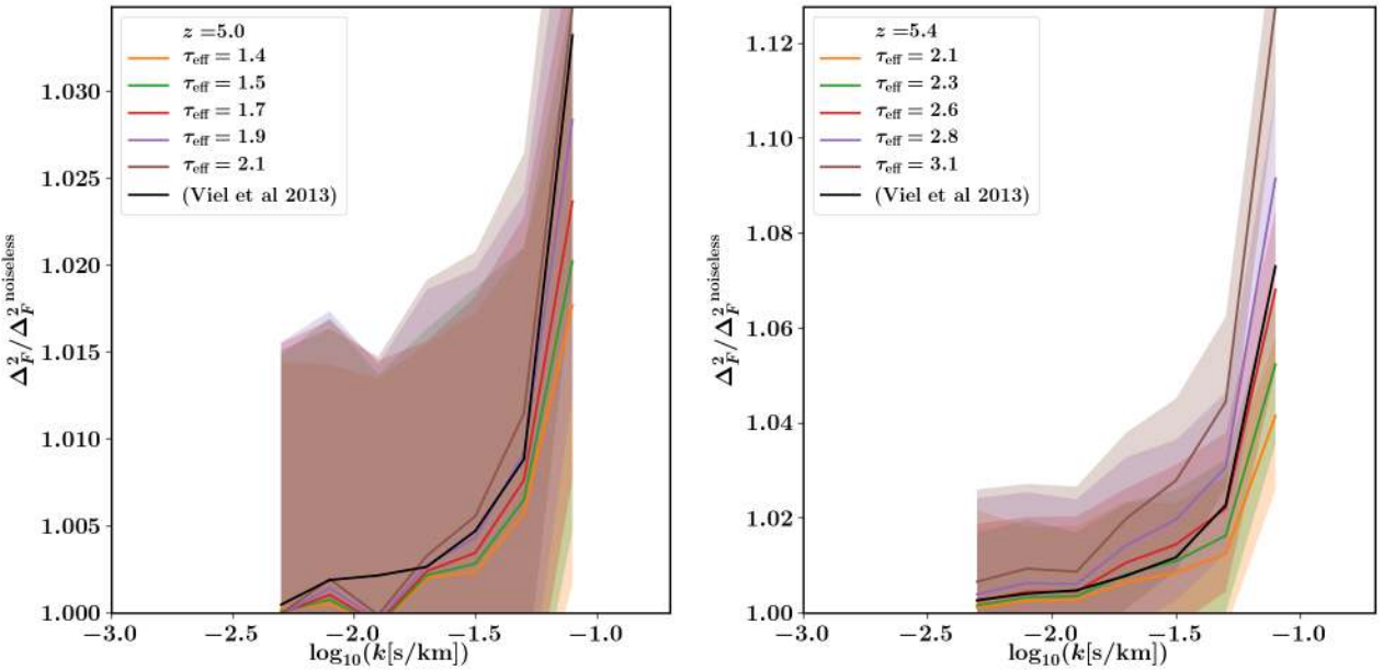
Figure C1. The effect of noise on FPS and its dependence from \tau_{\text{eff}} . We show the ratio between the FPS computed with and without noise. We have considered a signal-to-noise ratio equal to 15, for a CDM simulation without UVB, and with imposed temperature in post-processing equal to T = 2 \times 10^4 K. The left (right) panel regards the redshift interval centered on z = 5.0 ( z = 5.4 ). The solid lines refers to the mean of the ratio between the FPS computed with and without noise, the shaded region refer to the 1-\sigma uncertainty on the ratio. The black solid line is the correction for noise applied in Viel et al. (2013a), that is independent from \tau_{\text{eff}} . We conclude that the effect of noise depends on \tau_{\text{eff}} , and that accounting for noise only with a filter to the noiseless FPS is going to introduce a bias in the final estimate of the temperature.
