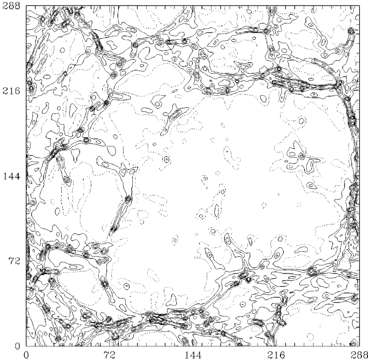
Figure 2 HI column density contours for a slice of the 10 h^{-1} Mpc (comoving) box from a cold dark matter model with a nonzero cosmological constant \Lambda ( \Lambda CDM) by Miralda-Escudé et al (1996).
