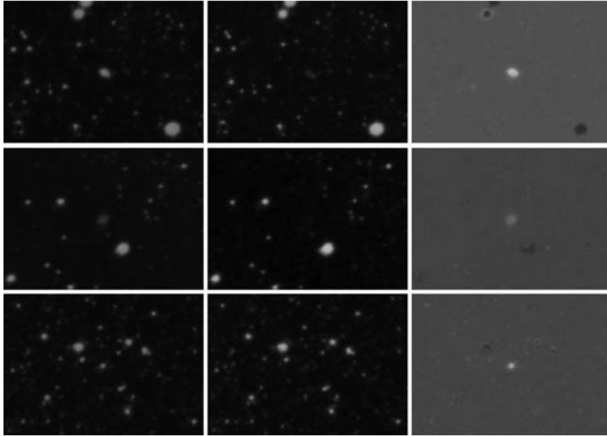
Figure 2. 1 \times 1.4 arcmin 2 extracts of SuperCOSMOS data around three newly discovered PNe in the Galactic bulge from the 3-h H \alpha survey data (a – left-hand column), matching 15 min Tech-Pan SR data (b – middle column) and difference image based on application of the PSF matching scheme of Bond et al. (2001) (c – right-hand column). This has proven to be particularly effective in uncovering a significant number of compact, new, bulge PNe (e.g. Peyaud 2005).
