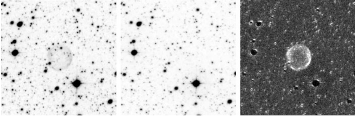
Figure 1. 4 \times 4 arcmin 2 extracts of SuperCOSMOS data around a newly discovered PN (PHR1520–5243) from the 3-h H \alpha survey data (a – left-hand panel), matching 15-min Tech-Pan short red SR data (b – middle panel) and simple quotient image (c – right-hand panel). The new PN is 53 arcsec in diameter and is only visible in the H \alpha image. Note the well matched depth for point sources between the two exposures and lack of an obvious central star candidate.
