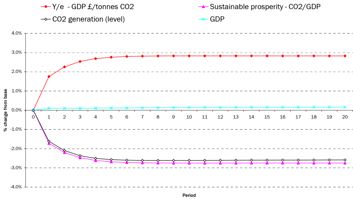
Figure 5.4 Impact on environmental indicators in response to a 5 per cent increase in energy efficiency in the UK
