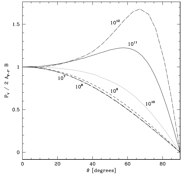
Fig. A.2. \theta -dependence of Eq. (A.1) for increasing emerging brightness temperature T_b\Delta\Omega (for [\Gamma + \Gamma_v] = 1 \text{ s}^{-1} ) from V02. The lines for T_b\Delta\Omega = 10^7 and 10^8 coincide and are the same as the lines for lower brightness temperatures. For fully unsaturated masers the dependence is equal to \cos\theta .
