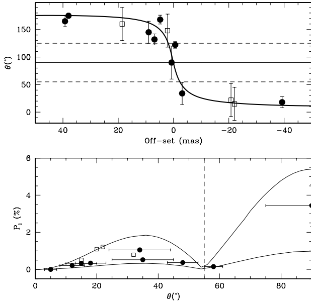
Fig. 10. ( Bottom ) The magnetic field angle \theta estimated from the fractional polarization P_1 measurement. The vertical dashed line indicates \theta_{\text{crit}} . The solid dots are the measured P_1 of the Field II maser features and the open squares are upper limits. The error bars in \theta are determined from the allowed range of \theta in the P_1 vs. \theta models of V06 shown for masers with emerging brightness temperatures T_b \Delta\Omega = 10^9 and 10^{10} K sr. (lower and upper solid line respectively). ( Top ) A model for the change of magnetic field angle \theta along the H 2 O maser filament. The thick solid line is the proposed model. The solid horizontal line indicates where the magnetic field direction changes. Between the dashed horizontal lines, which denote \theta_{\text{crit}} , the polarization vectors are perpendicular to the direction of the magnetic field. Above and below \theta_{\text{crit}} the polarization vectors are parallel to the magnetic field.
