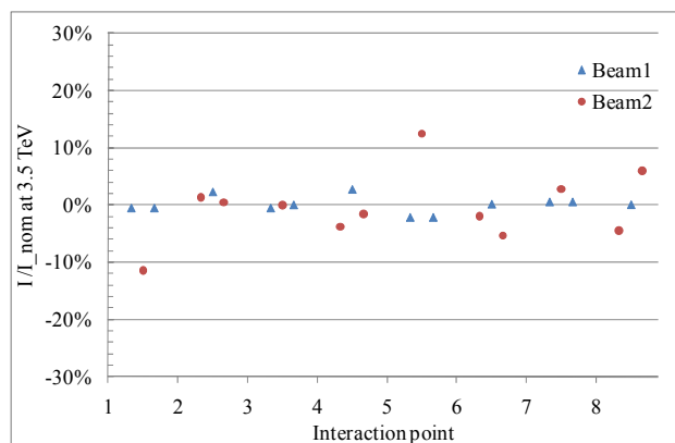
Figure 3: Used strength of skew quadrupoles at 3.5 TeV, w. r. t. nominal strength (April 1 st 2010, 18h15m).
