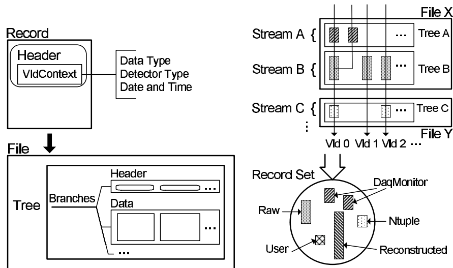
Fig. 43. MINOS data structure. The schematic on the left shows a MINOS record type derivation and header structure. The schematic on the right shows a MINOS stream as an ordered sequence of records stored in a ROOT TTree. On input, records stored in different streams are associated with each other by VldContext and not by Tree index.
