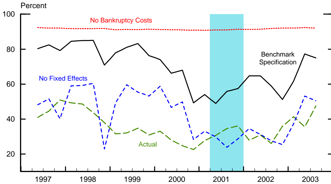
Figure 12: Model-Implied vs. Observed Recovery Rates
