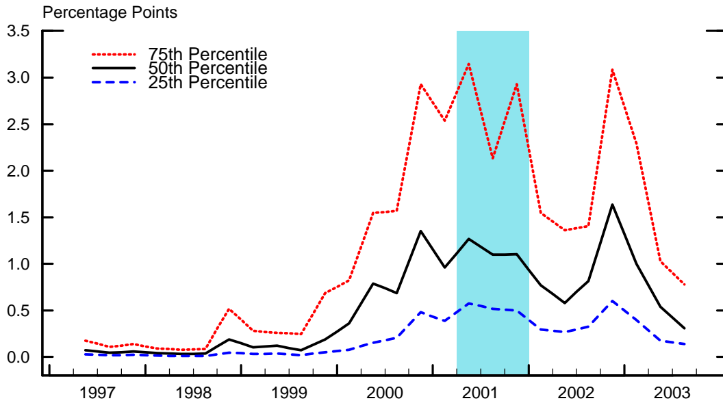
Figure 6: Cross-Sectional Distribution of the External Finance Premium
