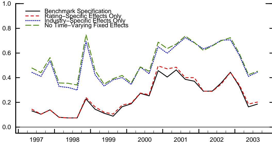
Figure 11: A Comparison of Estimates of the Bankruptcy Cost Parameter
