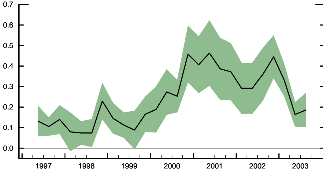
Figure 5: Benchmark Results for the Bankruptcy Cost Parameter
