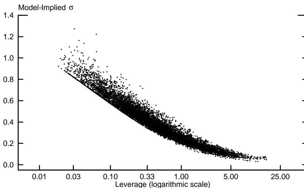
Figure 13: The Implied Relation between Leverage and Idiosyncratic Volatility
