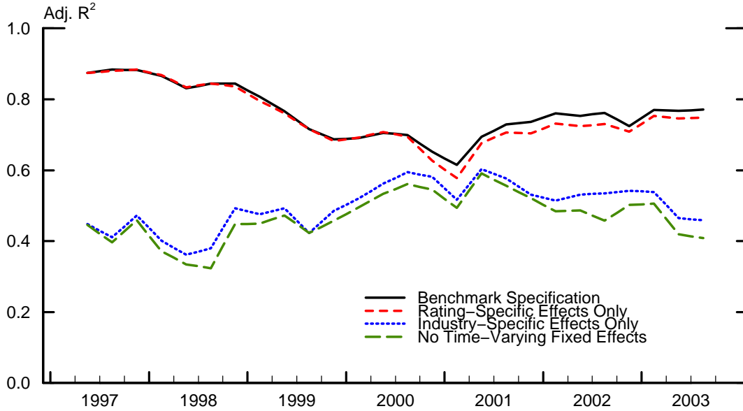
Figure 10: Goodness-of-Fit Comparison of Alternative Specifications
