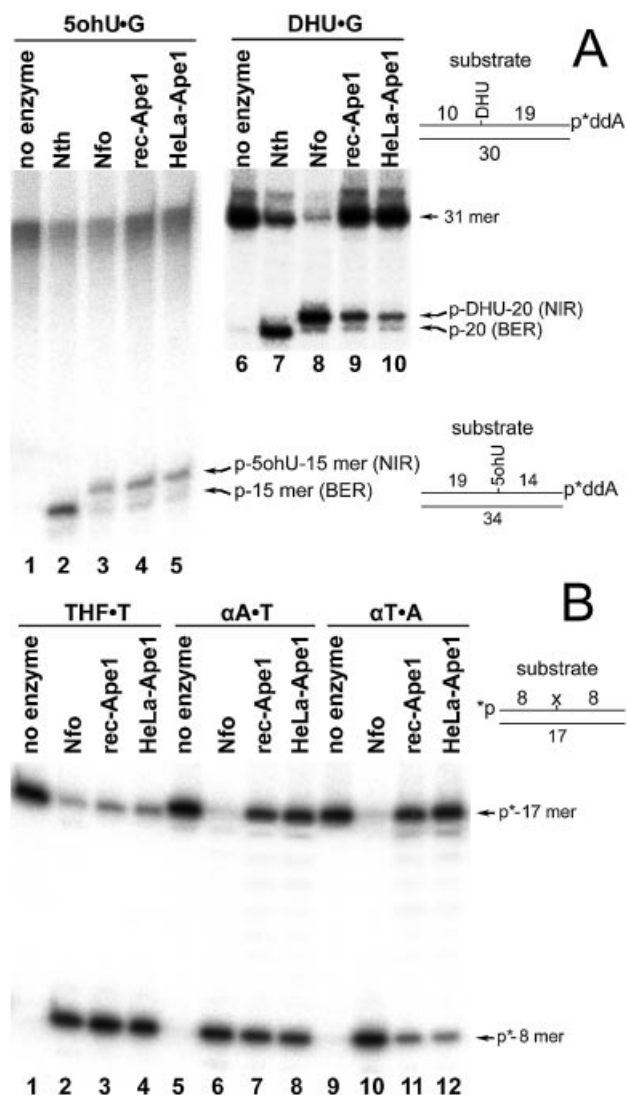
Figure 2. Comparison of substrate specificities of rec-Ape1 and HeLa-purified Ape1. Reactions were performed under standard NIR condition. (A) [ 3^{\prime} - ^{32} P]dCMP-labelled 5ohU-G and DHU-G; (B) 5^{\prime} - ^{32} P-labelled THF-T, \alpha A-T and \alpha T-A.
