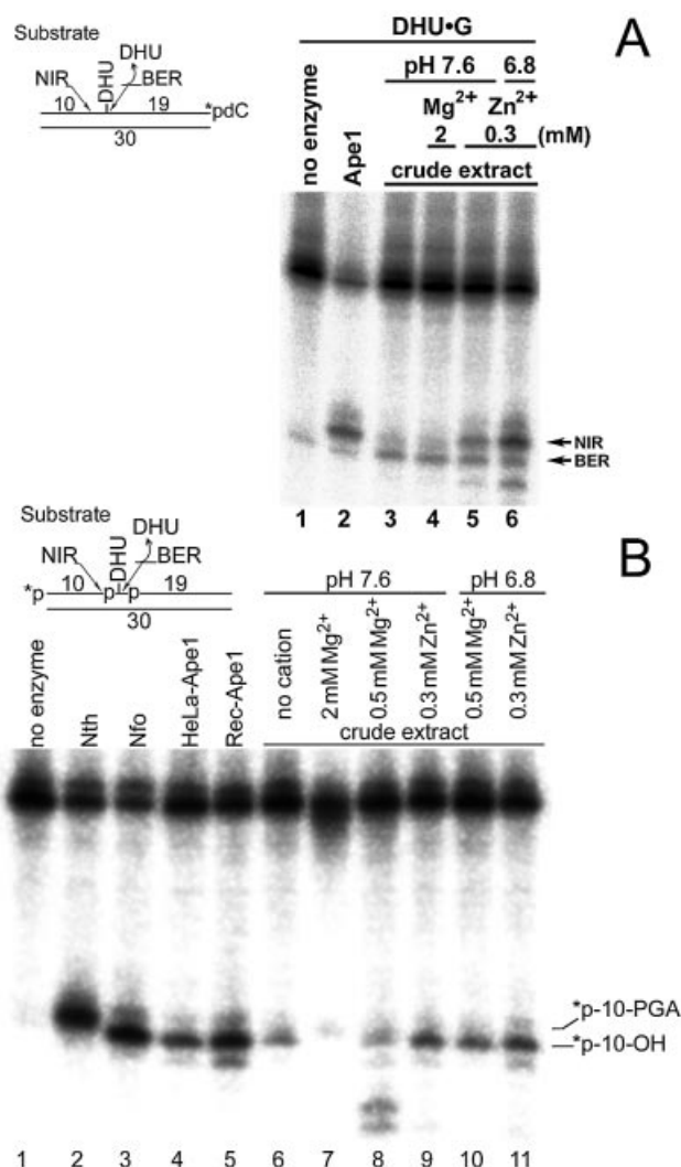
Figure 4. DNA repair assay using whole whole-cell extracts from HeLa cells. The extracts were incubated with 3'- (A) or 5'-labelled (B) DHU-G substrates under standard NIR or AP-endonuclease conditions with different concentrations of metal ions.
