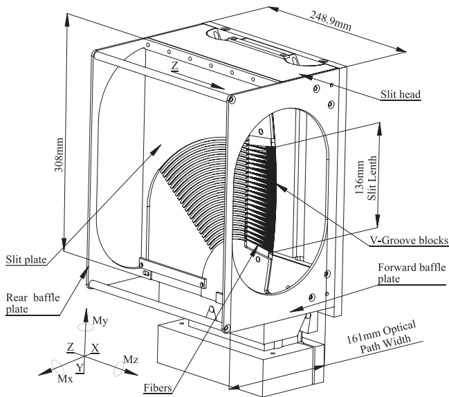
Figure 15. Schematic of slit plate installed on the cartridge slit head. The optical beam emanates from the fibers in the V-groove block in the positive Z direction, encounters the collimator mirror surface located 640.1 mm from the fiber faces, and is redirected back through the baffle plates toward the camera optics. The slit plate obscures 3.4% of the beam.
