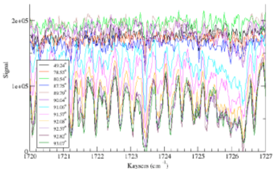
Fig. 6. Sunset solar occultation spectra acquired with the University of Denver Fourier transform infrared spectrometer in a region showing \text{HNO}_3 absorption lines. (P. Fogal, J. Olson, F. Murcray)
