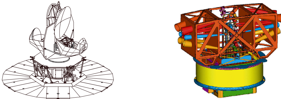
FIG. 1. — Left: A line drawing of the MAP satellite. Two back-to-back shaped Gregorian telescopes focus incident radiation onto the feeds which are located directly below the primary mirrors. The large circular disk at the bottom shields the telescopes from sunlight. The diameter of the disk is 5.1 m and the satellite is 3.6 m high. Right: The “focal plane assembly” (FPA) that houses the feeds. There are ten feeds on each side. The central area of the FPA houses the microwave receivers.
