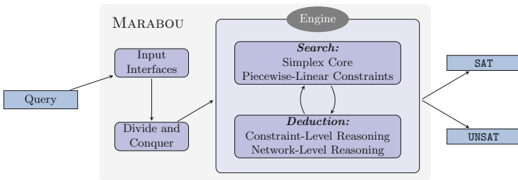
Fig. 1. The main components of Marabou.
