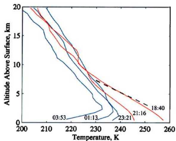
Figure 15. Temperature profiles from the southern hemisphere of Mars, obtained by Hinson et al. [1999] from MGS radio occultation measurements. Only the lower portion is shown to emphasize structure near the surface. Red and blue lines denote measurements made before and after sunset, respectively. The profiles show the nighttime development of a temperature inversion within \sim 3 km of the surface. Profiles were acquired over several months covering the seasonal interval 235^\circ \leq L_s \leq 342^\circ . The dashed line shows the adiabatic temperature gradient. Adapted from Hinson et al. [1999] with permission.
