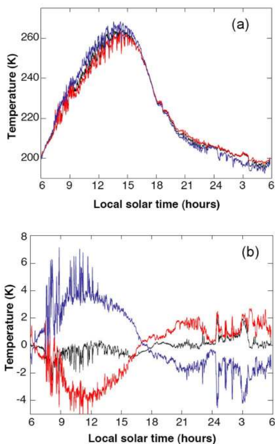
Figure 11. (a) The diurnal variation of atmospheric temperature measured by the top (red), middle (black), and bottom (blue) mast thermocouples at the MPF landing site, from 06:00 LST on sol 25 to 06:00 LST on sol 26. These thermocouples were 100, 50, and 25 cm, respectively, above the plane of the lander solar panels. Temperatures were sampled continuously at 4 s intervals throughout this period, but the plots use 30 point (2 min) running means for clarity (this smoothing reduces the amplitude and frequency of the fluctuations that are present in the raw data). (b) The data of Figure 11a plotted as temperature deviations from the mean of all three thermocouples. Sampling times and data smoothing are identical to those of Figure 11a. Adapted from Schofield et al. [1997] with permission of the American Association for the Advancement of Science.
