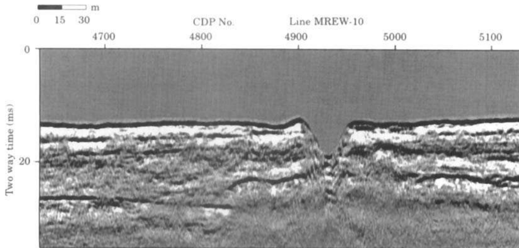
Figure 6. Processed portion of east-west orientated Chirp sub-bottom profile (acquired using a GeoAcoustics model 136A towed transducer system) MREW-10 showing a cross-section of the present day morphology of the excavation hole.
