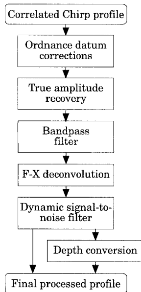
Figure 5. Flowchart of the sequence used in the seismic processing of the correlated Chirp data.
