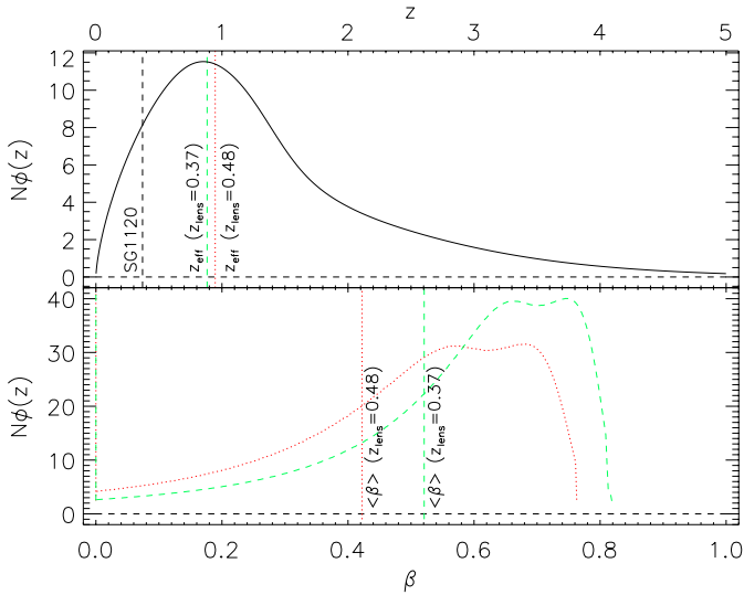
Fig. 6. Parametric redshift distribution of sources with i_{814} > 22 ( upper panel ) and the corresponding distribution in lensing efficiency \beta ( lower panel ). In the upper panel , the dashed green line corresponds to z_{\text{eff}} \approx 0.88 with respect to SG1120 and the dotted red line corresponds to z_{\text{eff}} \approx 0.95 with respect to the two structures at higher redshift. In the lower panel , the dashed green curve shows the distribution in \beta with respect to SG1120, with \langle \beta \rangle \approx 0.52 (dashed green vertical line), and the dotted red curve the distribution in \beta for the two structures at z = 0.48 , with \langle \beta \rangle \approx 0.42 (dotted red vertical line).
