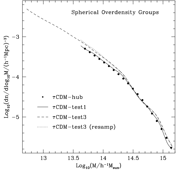
Figure A2. A resolution study of the effect of varying the particle mass on the mass function of SO halos. The dashed line shows the mass function obtained from \tau CDM-test3, and the solid line from \tau CDM-test1. These simulations have the same phases but differ by a factor of 8 in particle mass. The mass function is plotted for halos with 20 particles and above. The filled circles show the corresponding mass function in \tau CDM-hub which has the same particle mass as \tau CDM-test1. The dotted line shows the SO mass function when 1 in 8 particles are randomly sampled from \tau CDM-test3. This test shows that the SO mass function is sensitive to the particle mass, unlike the FOF mass function in Fig. A1.
