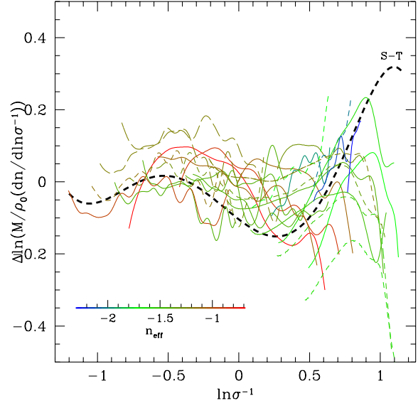
Figure 8. The residual between the fitting formula, eqn. 9, and the FOF(0.2) mass functions for all the simulation outputs listed in Table 2. The lines are colour codes according to the value of n_{\text{eff}} . Solid lines correspond to simulations with \Omega = 1 , short dashed lines to flat, low \Omega_0 models, and long dashed lines to open models. The heavy dashed line shows the Sheth-Tormen formula (equation (7))
