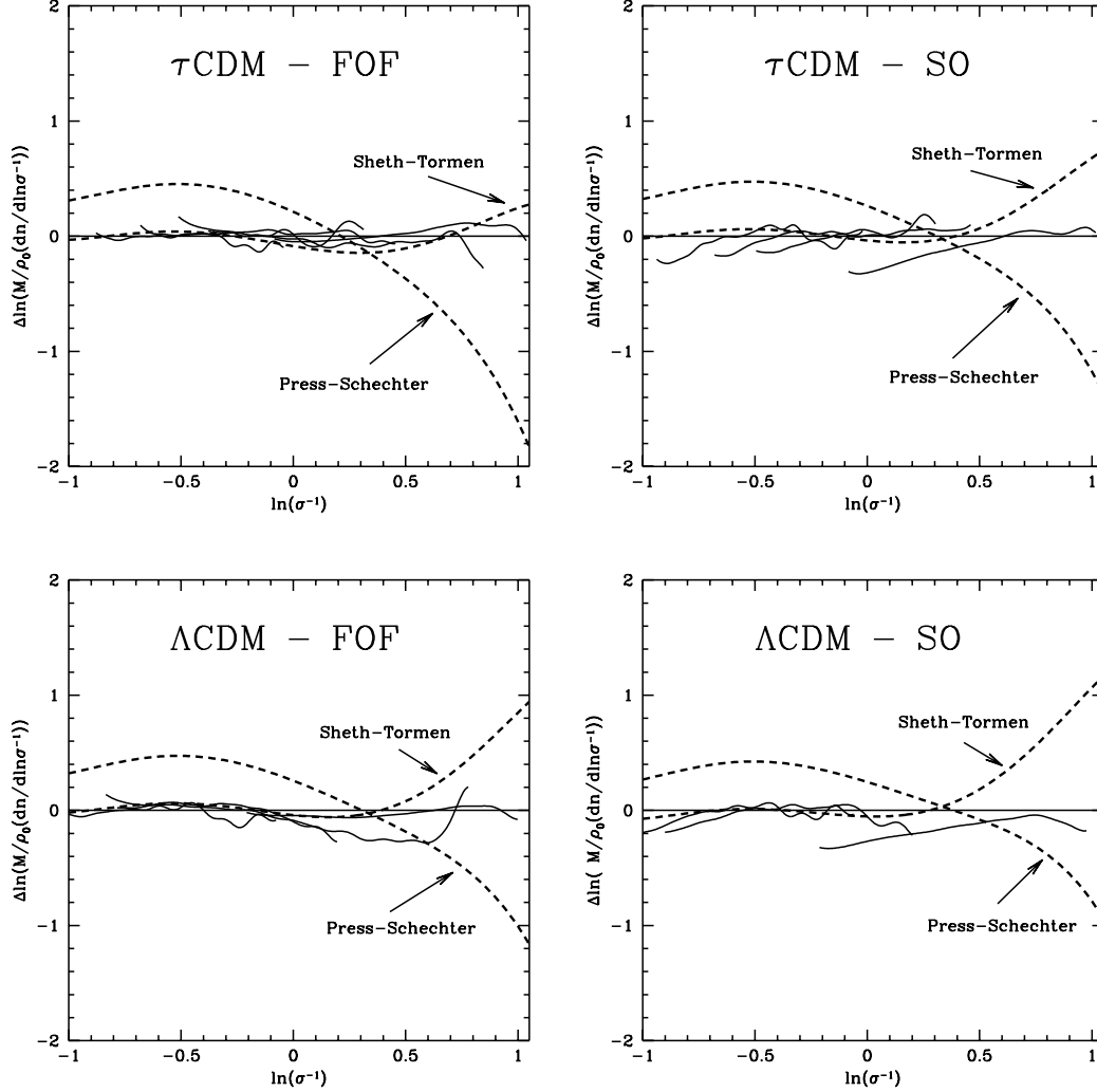
Figure A3. The residuals between the fitting formulae for the mass function given in appendix B and (i) the simulations (solid lines) and (ii) the Press-Schechter and Sheth-Tormen models (dashed lines.) The simulation curves are plotted up to the point where the fractional Poisson error reaches 10%. The simulations themselves can be seen to be mutually consistent at about the 10% level although the differences are, for the most part, larger than the Poisson errors. The P-S curve shows an excess at low masses and a deficit at high masses. The Sheth-Tormen mass function fits the low mass end well, but overestimates the number of high mass clusters. Note that we use natural logarithms in this plot.
