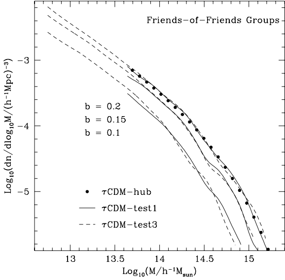
Figure A1. A resolution study of the effect of varying the particle mass on the mass function of FOF halos for three values of the linking parameter, b . The dashed lines show the mass functions obtained from \tau CDM-test3, and the solid lines from \tau CDM-test1. These simulations have the same phases but differ by a factor of 8 in particle mass. The mass function is plotted for halos with 20 particles and above. The filled circles show the corresponding mass function in \tau CDM-hub which has the same particle mass as \tau CDM-test1. Defined in this way, the mass function is remarkably robust.
