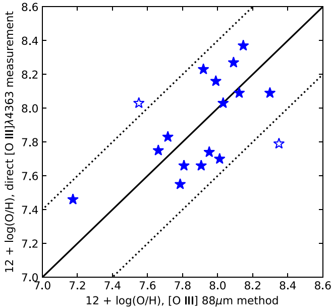
Figure 1. Comparison of 12 + \log(\text{O}/\text{H}) determined from [\text{O III}] 88 \mu\text{m} and SFR, compared to measurements based on standard optical emission line methods (using [\text{O III}] \lambda 4363 as a T_e diagnostic). Blue stars show all galaxies with suitable [\text{O III}] 88 \mu\text{m} measurements from Herschel taken as part of the Dwarf Galaxy Survey (DGS). The DGS sample probes subsolar metallicities relevant for comparison to high-redshift galaxies (here we adopt a solar abundance 12 + \log(\text{O}/\text{H}) = 8.69 ). The solid black line shows the one-to-one relation, with dashed lines at \pm 0.4 dex (corresponding to 2\sigma scatter of the solid symbols), demonstrating reasonably good agreement. We note that the dashed lines serve to illustrate scatter about the one-to-one relation and are not intended to represent confidence intervals. The galaxies that differ by >0.4 dex (open symbols) can be reconciled with direct measurements as discussed in the text.
