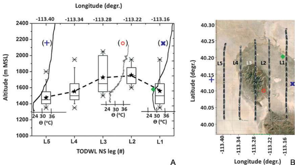
FIG. 9. (a) Box-and-whisker plot of CBL heights derived from aerosol backscatter profiles along the (b) north-south TODWL flight legs. The data were collected during a morning mission between 1012 and 1052 MDT 10 Oct 2012. The horizontal line in the box and the bottom and top lines of the box show the median of the data and the lower and upper quartiles (25% and 75%), respectively. The whiskers show the minimum and maximum values while * is the mean value. Potential temperature profiles from the radiosondes at the Playa (+) and Sagebrush (x) sites, a DATAHAWK UAV (O) profile near the ES-2 tower, and the CBL height based on FM-CW radar (♦) are shown in (a).
