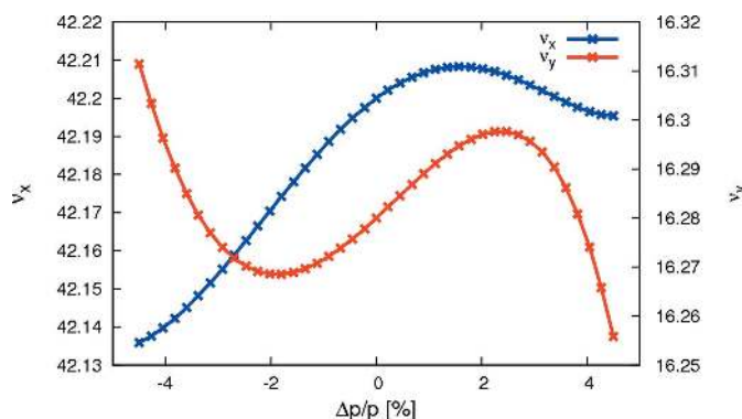
Figure 5 Chromaticity in the MAX IV 3 GeV storage ring (Leemann, 2012d).
