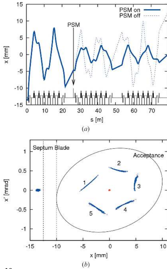
Figure 10 Top: trajectory of the injected bunches in the MAX IV 3 GeV storage ring starting at the septum (Leemann, 2012b). The PSM is installed in the second long straight and kicks the injected bunch into the ring acceptance. Bottom: tracking of injection and capture of 1000 particles at the septum in the 3 GeV storage ring. The first five turns are indicated in blue. For comparison, the stored beam is indicated in red.
