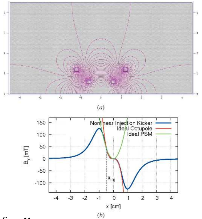
Figure 11 Upper half geometry (top) and resulting field profile in the midplane (bottom) of a BESSY-type non-linear injection kicker adapted to the MAX IV 3 GeV storage ring (Leemann & Dallin, 2013). Note that the resulting field around the centre is similar to an octupole.
