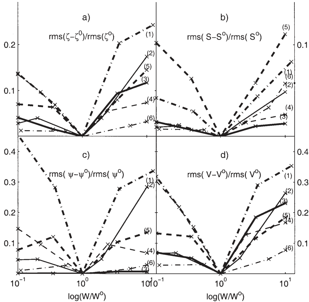
Fig. 12 Dependence of the SSH field (a); salinity field (b); transport function (c) and; velocity field on 25 m on relative changes in the value of covariance functions W_\zeta^s - SSH smoothness, curve (1); W_\zeta - corresponding to "SSH data" (2); W\psi - smoothness of total transport function (3); W_S^s - temperature and salinity smoothness (4,5); W_S - corresponding to salinity data (6).
