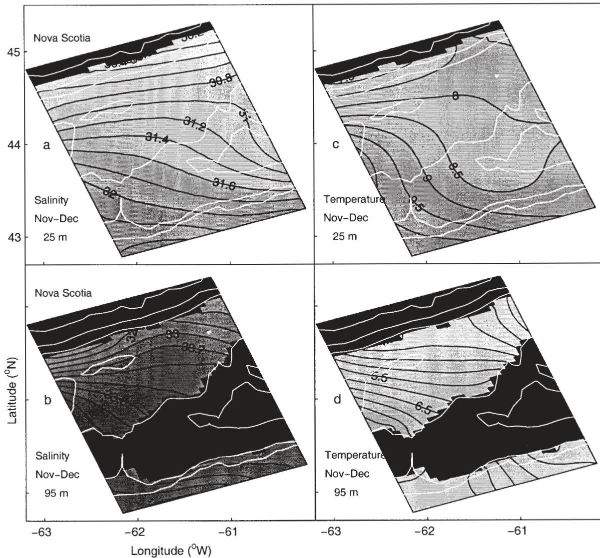
Fig. 5 Optimized salinity (a,b) and temperature (c,d) fields at 25 and 95 m for the fall period.
