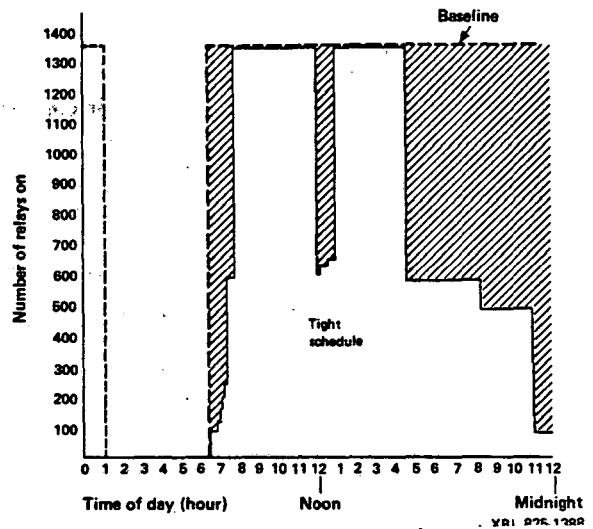
Fig. 5. Lighting load using tight schedule (World Trade Center).
