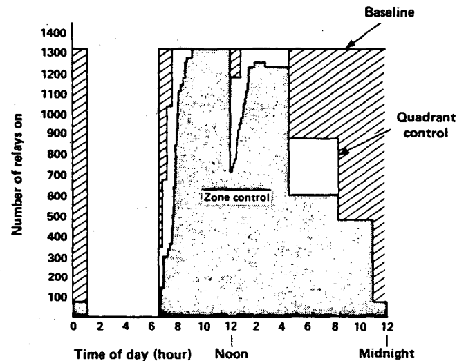
Fig. 7. Effect of different switching zone sizes on lighting load profile for manual-on/automatic-off operation (World Trade Center).
