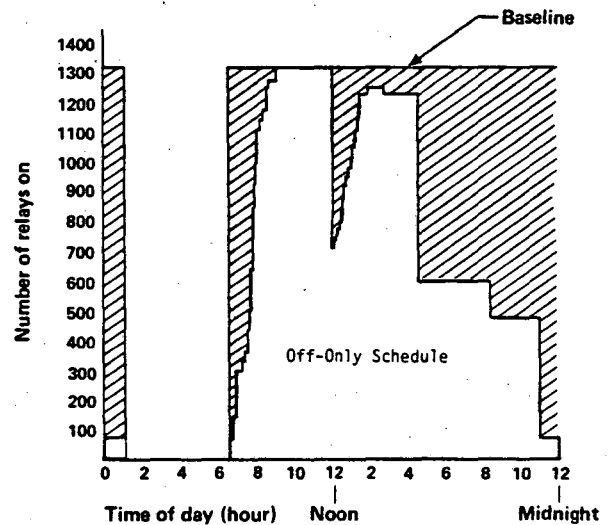
Fig. 6. Lighting load profile for manual-on/automatic-off operation (World Trade Center).
