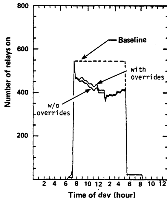
Fig. 9. Effect of daylight-activated switching on lighting loads in daylight areas averaged over eight weekdays in March
