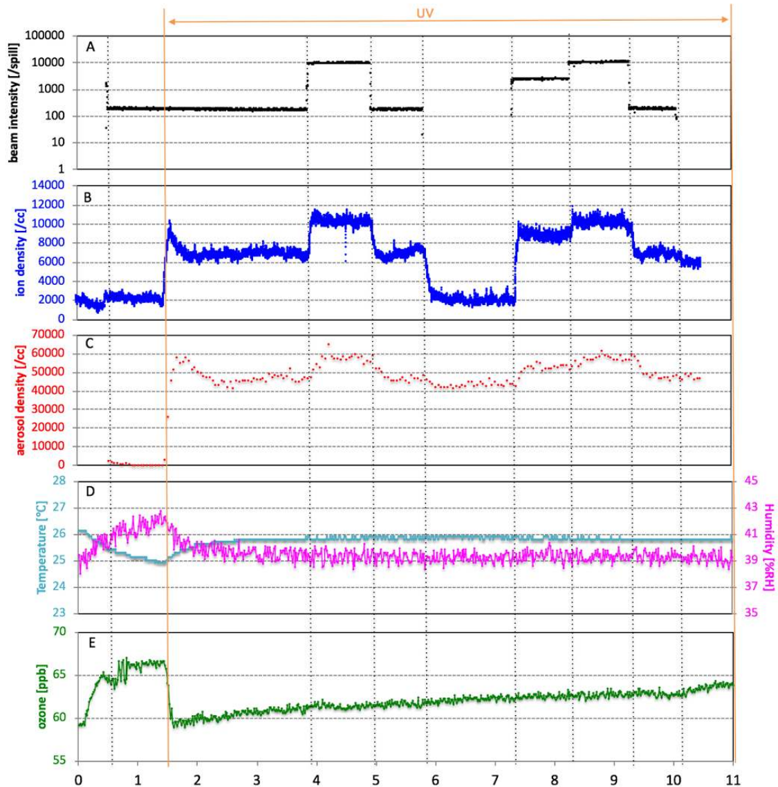
Fig. 2: Temporal variation of (A) beam intensity, (B) ion density, (C) aerosol density, (D) temperature and RH, and (E) ozone concentration in the chamber during RUN2. The x-axis indicates the elapsed time, where 0 s is defined as the time the measurement started. The vertical black dotted lines indicate the time when the beam intensity was changed. The vertical orange lines indicate the time interval of UV irradiation.
