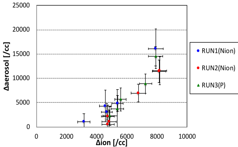
Fig. 3: Relationship between the \Delta aerosol and the \Delta ion for N ion beam (blue and red circles, respectively) and proton beam (green triangles).
