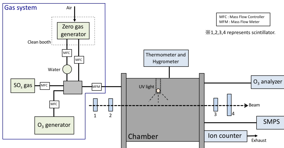
Fig 1: Diagram of the chamber system.
