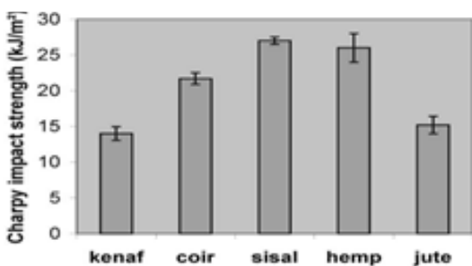
Fig7: charpy impact strength of fibre reinforced polymer composites [19]
