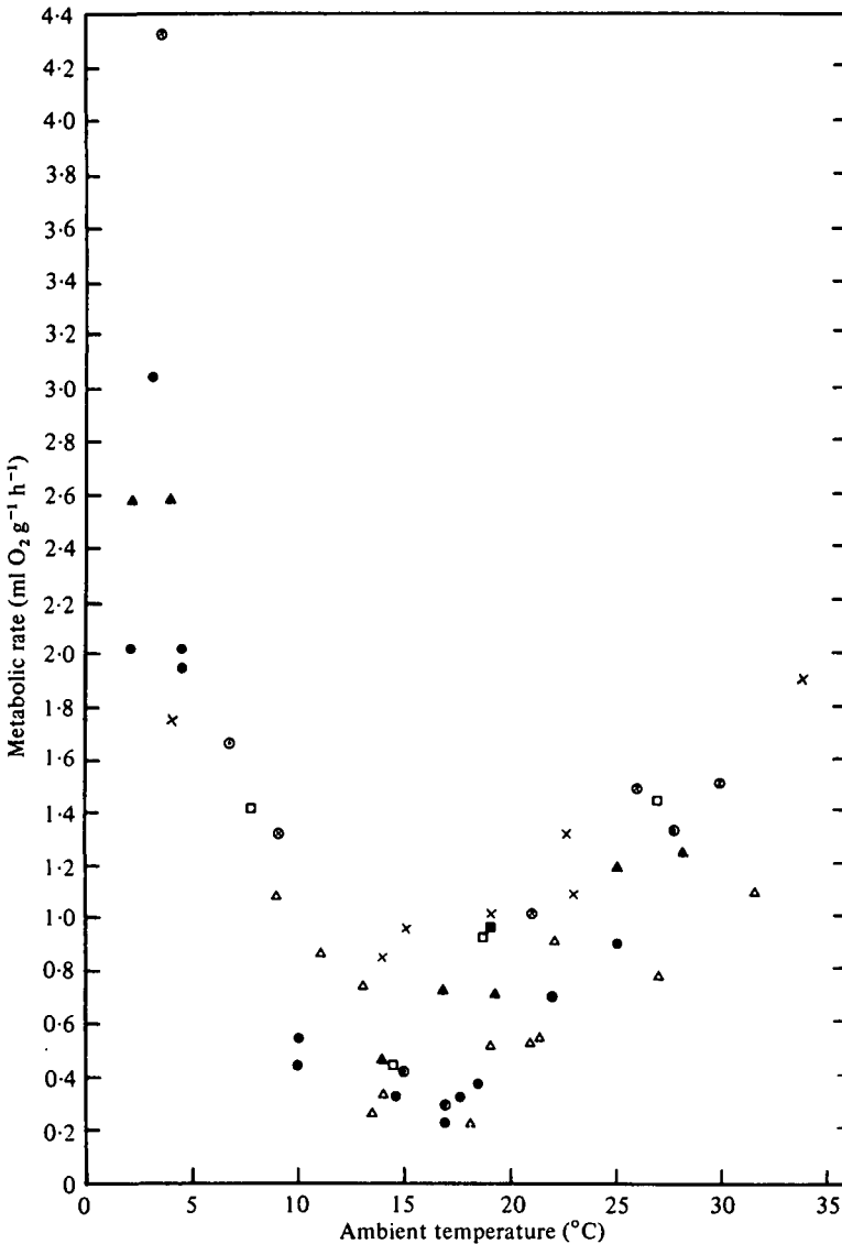
Fig. 9. Metabolic rates of eight different swarms with different numbers of bees (□, 1800; ■, 4900; ●, 5280; ▲, 5650; ○, 8200; △, 10 000; ⊗, 15 300 and, ×, 16 600) as a function of ambient temperature. All of these swarms had been at rest for at least 8 h. None had been fed. All had been maintained in the temperature-controlled room.
