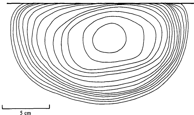
Fig. 7. Temperature isotherms in a clump of 7000 dead bees after they had been heated uniformly throughout to 44 °C, and then allowed to cool at T_A = 3 °C. Core temperature after 140 min was 22 °C (this figure). Each line represents at 1 °C temperature isotherm.
