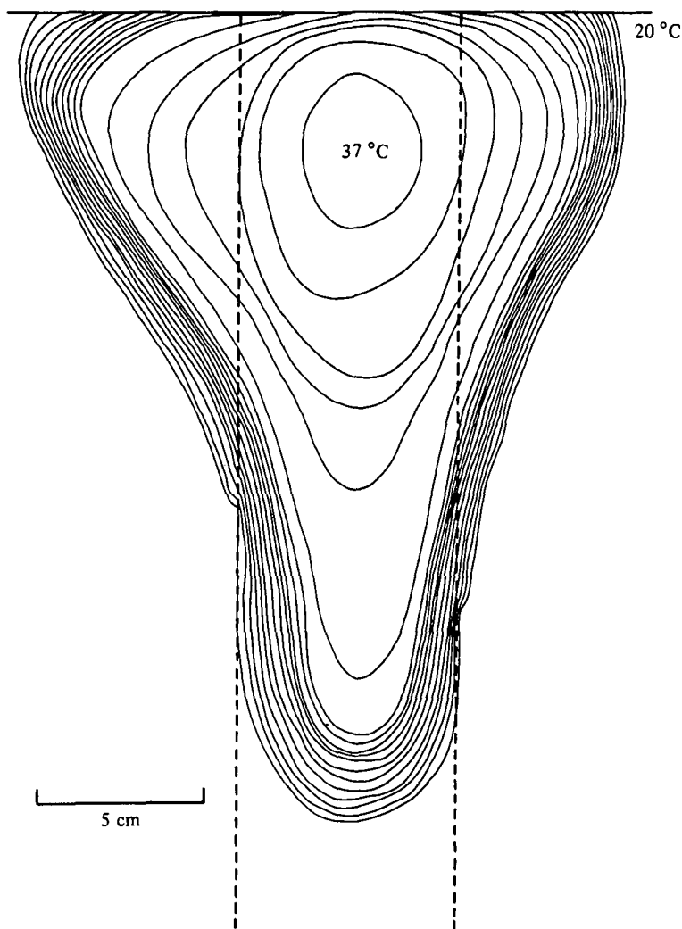
Fig. 19. Temperature isotherms ( 1\text{ }^{\circ}\text{C} ) in a swarm of 8000 bees that is partially built in a gauze cylinder attached to the plexiglass foothold of the swarm. T_A = 4\text{ }^{\circ}\text{C} .
