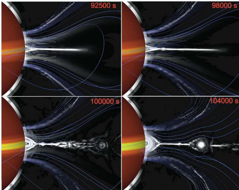
Figure 13. Close-up view of photospheric B_\phi (red/yellow contours on the solar surface), normalized current density R_s|J|/c in the r - \theta plane (grayscale), and magnetic field lines (blue) in the simulation during the impulsive flare phase. The frame-to-frame variations in B_\phi on the solar surface are explained in the first discussion of Fig. 3. The temporal evolution is shown in the movie available in the electronic edition (movie2.mpg). As in Fig. 3, the minimum B_\phi (dark red) is zero; the maximum value (yellow) is saturated at 2 G. The minimum value of R_s|J|/c (black) is effectively zero; the maximum (white) is saturated at 0.2 G.
