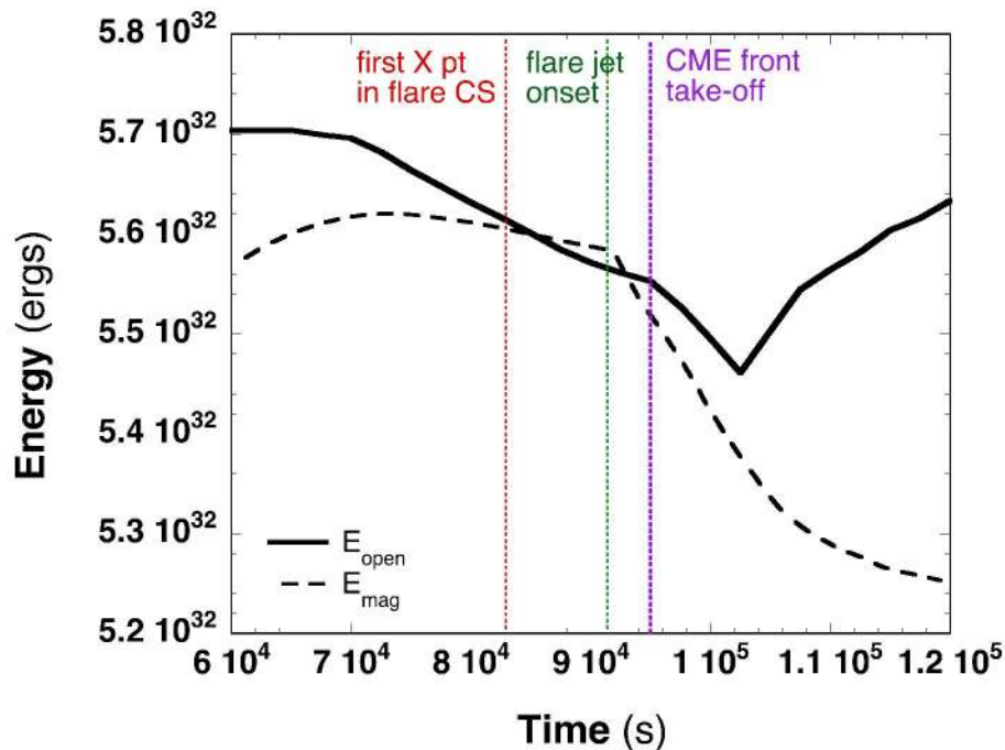
Figure 16. Volume-integrated magnetic energy ( E_{mag} ) and partially open energy ( E_{open} ) in the middle of the breakout simulation. Key times are marked by dotted vertical colored lines
