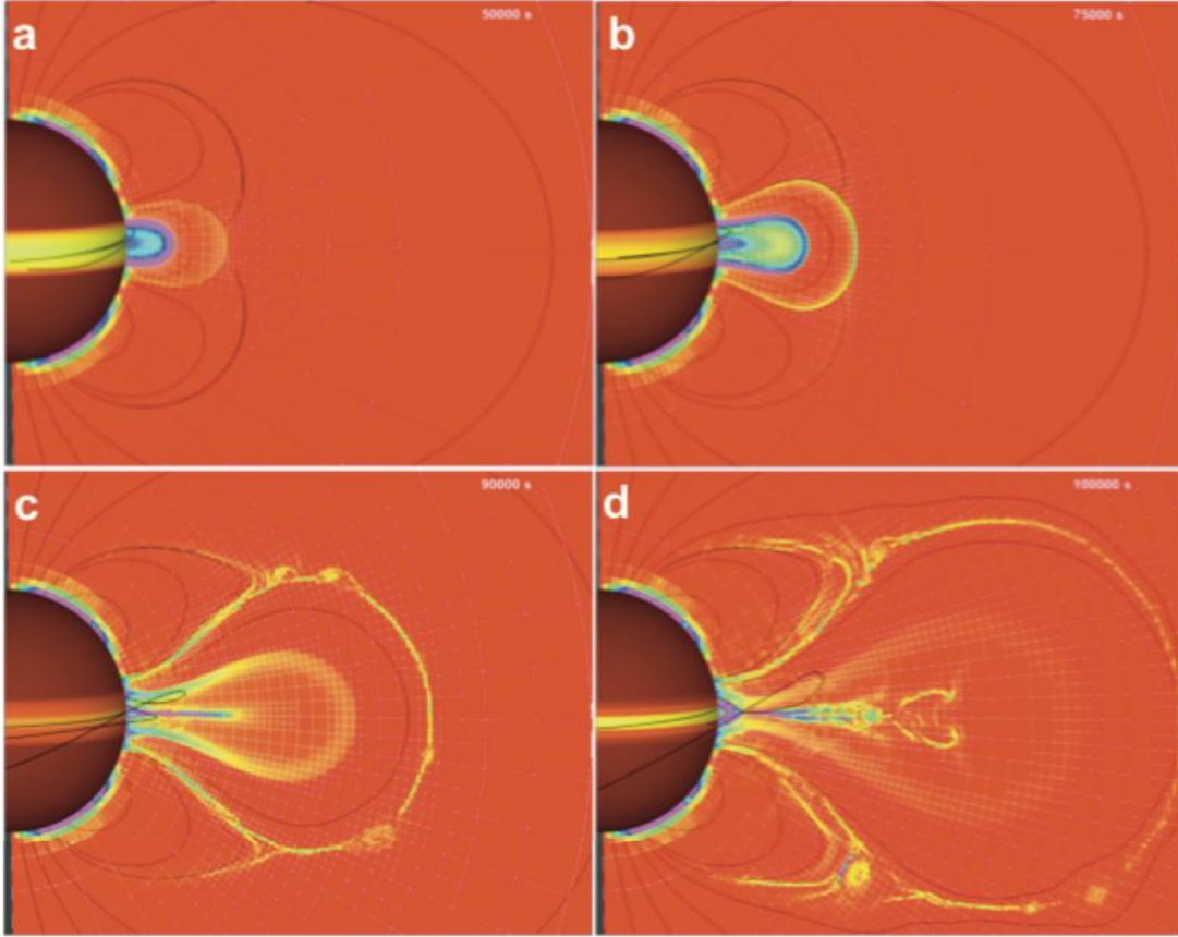
Figure 3. Photospheric B_\phi (red-yellow contours on the r=R_s surface), normalized current density magnitude R_s|J|/c in the r - \theta plane (red to magenta), grid blocks (white lines), and magnetic field lines (black) in the simulation at selected times. a) 50,000 s. b) 75,000 s. c) 90,000 s. d) 100,000 s. The full temporal evolution is shown in the movie available in the electronic edition (movie1.mpg). The minimum B_\phi (dark red) is zero; the maximum value (yellow) is saturated at 2 G. The minimum value of R_s|J|/c (red) is zero; the maximum value (magenta) is saturated at 0.2 G.
