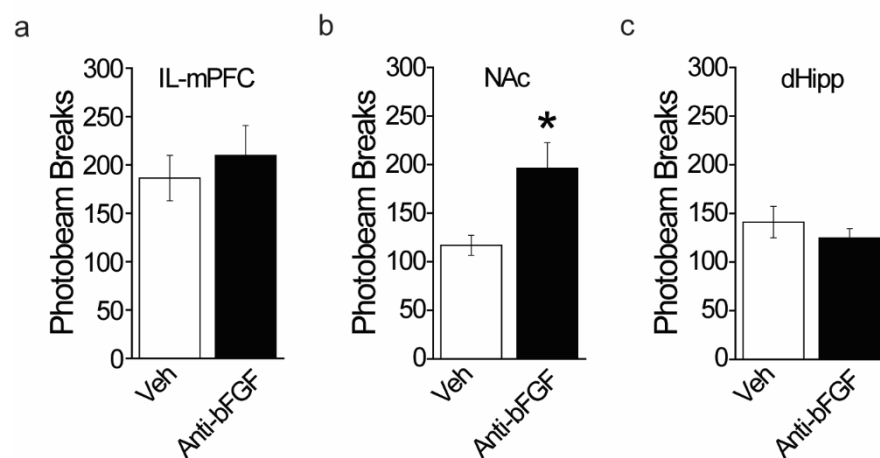
Figure 22: Neutralizing bFGF in IL-mPFC and dHipp does not affect locomotion, but does in NAc. (a) Neutralizing bFGF in IL-mPFC does not affect locomotion. (b) Neutralizing bFGF in NAc increases
