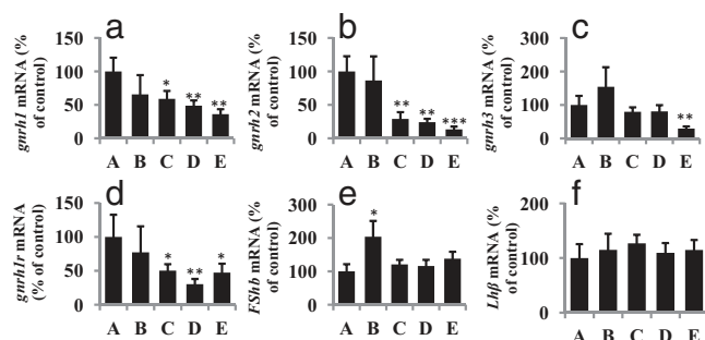
Figure 1. The effect of chronic treatment of Kiss1 and Kiss2 peptides on brain and pituitary mRNA levels of major reproductive axis genes (a) gnrh1 , (b) gnrh2 , (c) gnrh3 , (d) gnrh1r , (e) FShβ , and (f) Lhbβ . mRNA levels were measured in dummy-run female striped bass treated for 10 weeks with EVAc implants containing, respectively, (A) no peptide (n = 8), (B) pyroGluKiss1-15, 25 \mu\text{g}/\text{kg} BW (n = 11), (C) pyroGluKiss1-15, 75 \mu\text{g}/\text{kg} BW (n = 12), (D) Kiss2-12, 25 \mu\text{g}/\text{kg} BW (n = 12), and (E) Kiss2-12, 75 \mu\text{g}/\text{kg} BW (n=11). Results are presented as mean \pm SEM of % of control levels obtained from the absolute copy number of mRNA of each gene. Statistical difference was accepted when P \leq .05 . *, P \leq .05 ; **, P \leq .01 ; ***, P \leq .005 .
