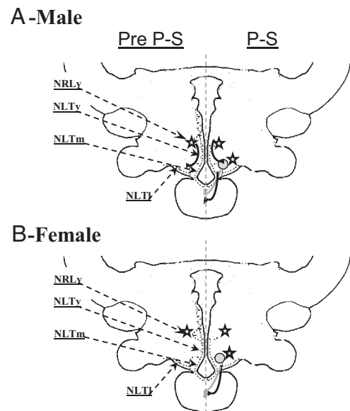
Figure 8. Schematic illustration summarizing the changes in the distribution of kiss1 and kiss2 neurons and their projections in the NLT and NH before and immediately before spawning. A, Male. B, Female. Gray circle and lines denote kiss1 neuronal soma and axons, respectively. The 2 hemispheres of the brain (the optic tectum above the hypothalamus is not shown) are divided by a gray dashed line, in which the hemisphere on the left represents reproductive stages before the prespawning phase (Pre P-S) and the hemisphere on the right represents the prespawning stage (P-S). Black stars represent either neuronal soma or axon terminal bundles, black lines denote Kiss2 axonal projections. P, pituitary.
