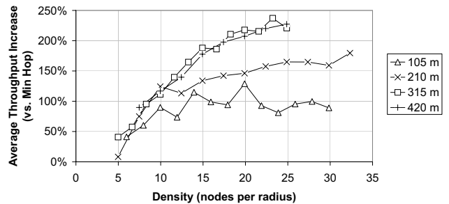
Figure 8: Average throughput increase of MTM along a randomized straight line path.
