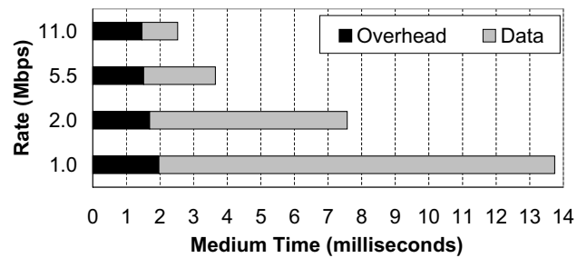
Figure 3: Medium Times for 802.11b Transmissions
