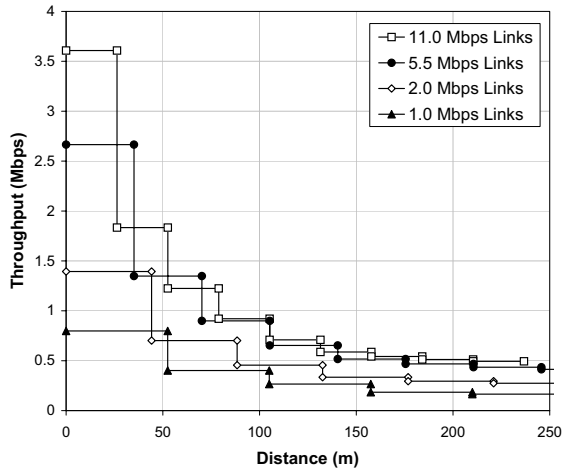
Figure 6: Throughput Loss Along a Path
