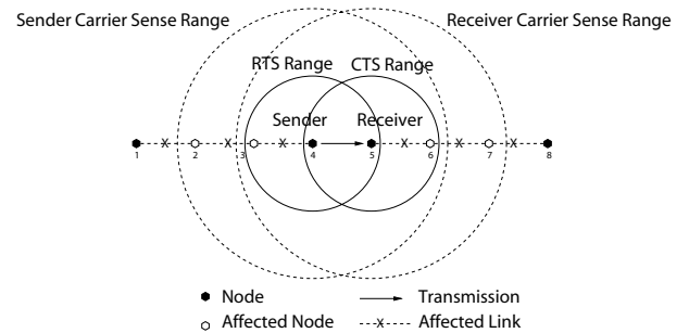
Figure 5: Effect of Transmission on Other Nodes
