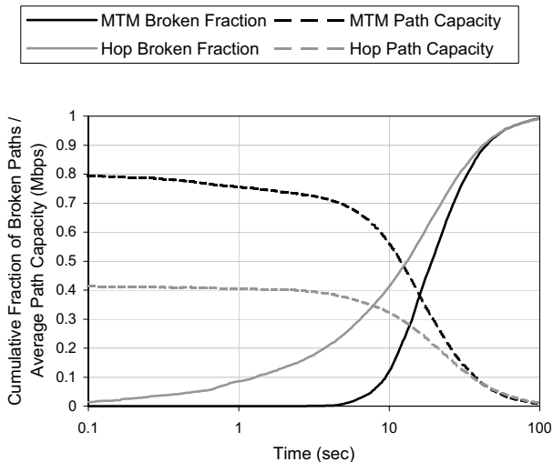
Figure 7: Path Elasticity Results
