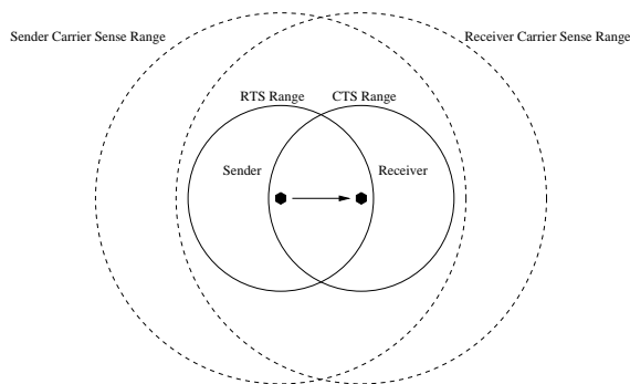
Figure 2: 802.11 Communication
