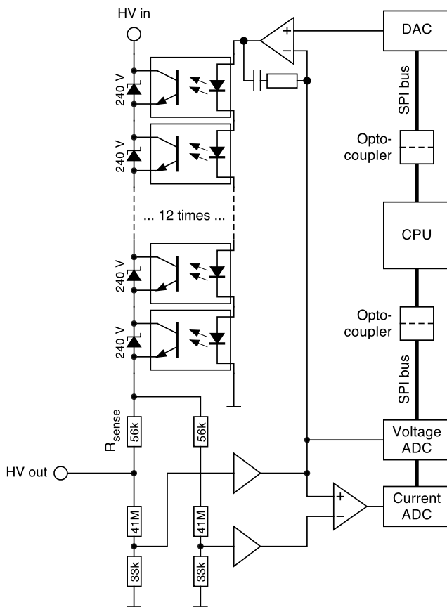
Fig. 85 Simplified schematics of the high-voltage regulator. The 240 V Zener diodes protect the optocouplers, so that no more than 240 V drop across the transistors of the optocouplers
