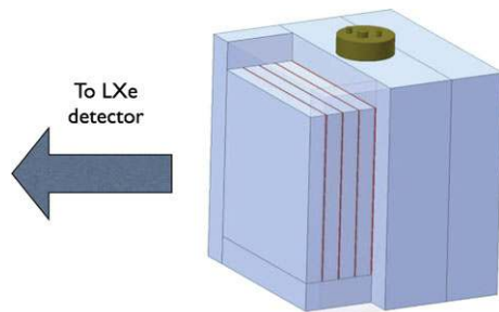
Fig. 62 The nickel slabs (red), moderator (blue) and neutron generator (green) (Color figure online)
