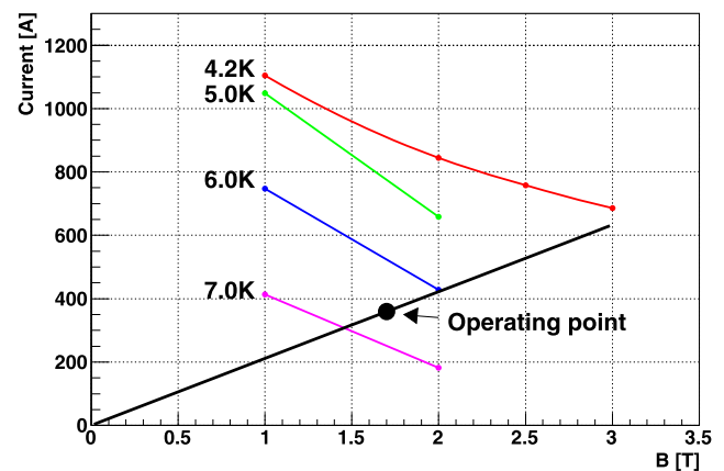
Fig. 18 Measured critical current of the conductor as a function of the applied magnetic field. The operating condition of COBRA is also shown
