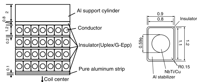
Fig. 17 Layer structure of the central coil (left) and the cross-sectional view of the conductor (right). Units in mm
