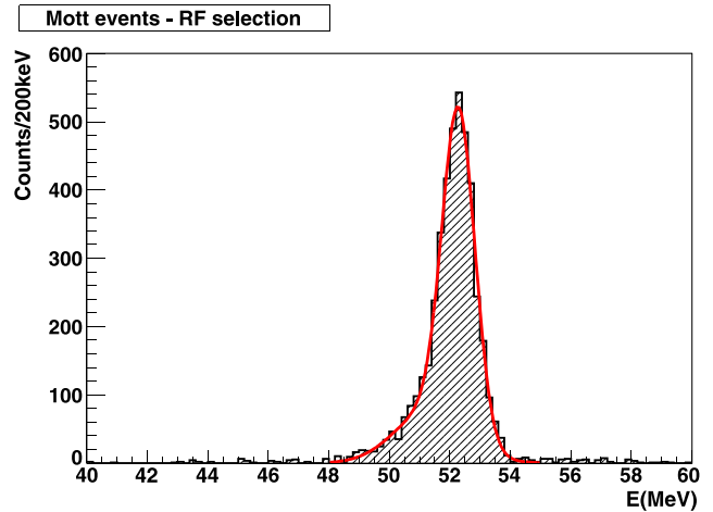
Fig. 66 The momentum distribution of RF-selected Mott events
