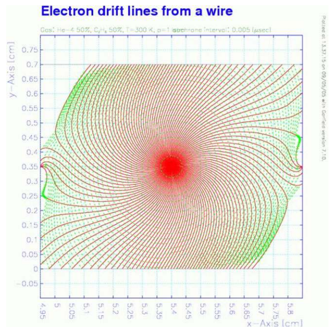
Fig. 23 Isochrons (dashed green) and drift (solid red) lines of a cell with B = 1.60 T (Color figure online)
