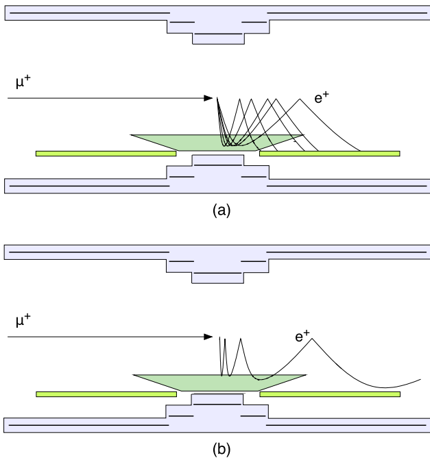
Fig. 13 Concept of the gradient magnetic field of COBRA. The positrons follow trajectories at a constant bending radius weakly dependent on the emission angle \theta (a) and those transversely emitted from the target ( \cos\theta \sim 0 ) are quickly swept away from the DCH (b)
