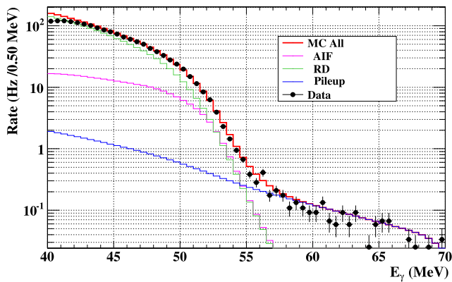
Fig. 90 Inclusive \gamma -ray spectrum in LXe. Data (dots) and MC (lines). MC spectrum is separated into contributions from AIF, RMD and pile-up from multiple \gamma -rays
