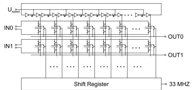
Fig. 78 Simplified schematics of the inverter chain of the DRS4 chip
