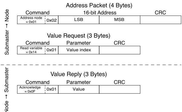
Fig. 83 Typical communication protocol example between a submaster and a node
