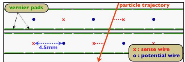
Fig. 22 Schematic view of the cell structure of a DCH plane
