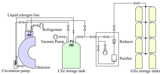
Fig. 51 Schematic view of LXe storage and purification systems as well as of the detector
