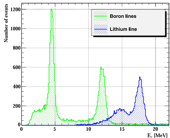
Fig. 69 Measured calibration lines from the reactions ^{11}\text{B}(p, \gamma_{4.4}\gamma_{11.6})^{12}\text{C} (green) and ^7\text{Li}(p, \gamma_{17.6})^8\text{Be} (blue) (Color figure online)
