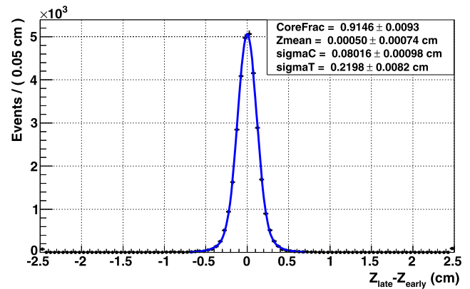
Fig. 31 A fit to the distribution of the difference of projected z coordinates for two-hit clusters
