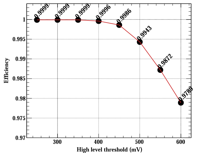
Fig. 45 DTD efficiency vs. high threshold value. The efficiency plateau is reached for \text{HT} \leq 400 mV
