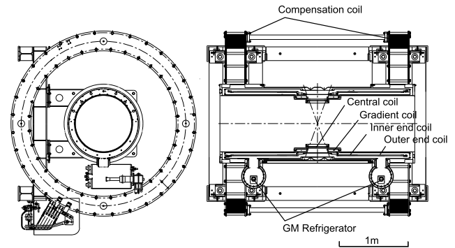
Fig. 15 Cross-sectional view of the COBRA magnet
