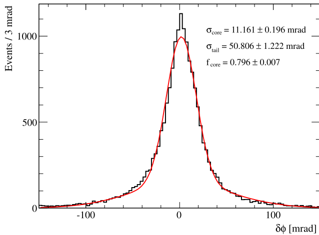
Fig. 33 A fit to the distribution of \delta\phi_e \equiv \phi_e^{\text{1st turn}} - \phi_e^{\text{2nd turn}} on double-turn events. The distribution is fitted with a double Gaussian function convolved with itself, and the corresponding core and tail widths are shown, along with the fraction of events in the core component
