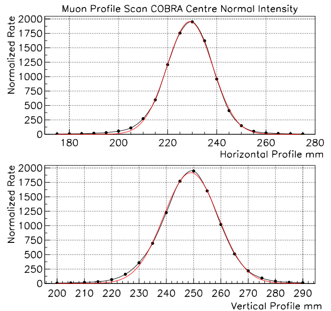
Fig. 7 Scanned horizontal and vertical muon beam-spot profiles measured at the centre of COBRA. The red lines show the Gaussian fits to the distributions that yield \sigma_{x,y} \sim 10 mm and a total stopping intensity of \sim 3 \times 10^7 \mu^+/s at a proton beam intensity of 2.2 mA and momentum-bite of 5.0 % FWHM (Color figure online)
