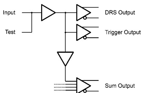
Fig. 80 Block diagram of a splitter channel for the LXe detector
