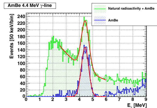
Fig. 61 The AmBe \gamma -ray spectrum measured by the LXe detector. A Gaussian and exponential fit is superimposed on the green spectrum. A Gaussian fit is used after subtracting the exponential natural radioactivity background
