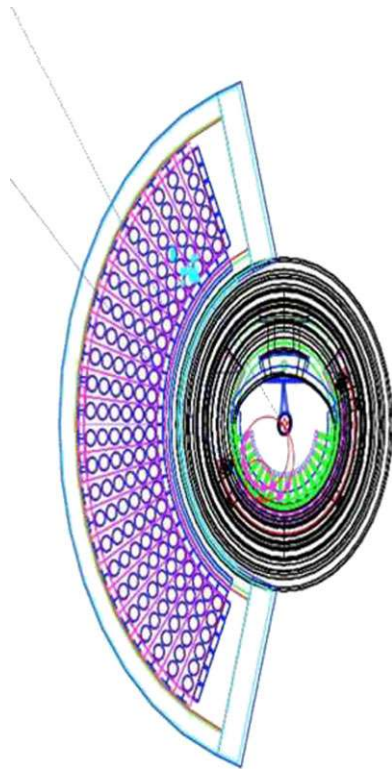
Fig. 87 A simulated event \mu^+ \rightarrow e^+ \gamma
