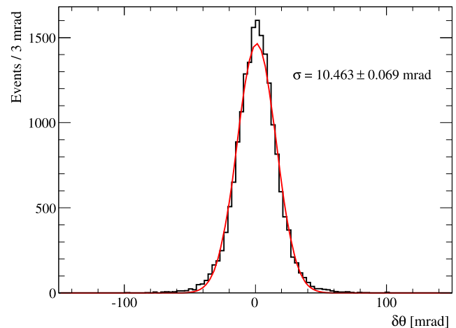
Fig. 32 A fit to the distribution of \delta\theta_e \equiv \theta_e^{\text{1st turn}} - \theta_e^{\text{2nd turn}} on double-turn events. The distribution is fitted with a single Gaussian convolved with itself, and the corresponding width is shown
