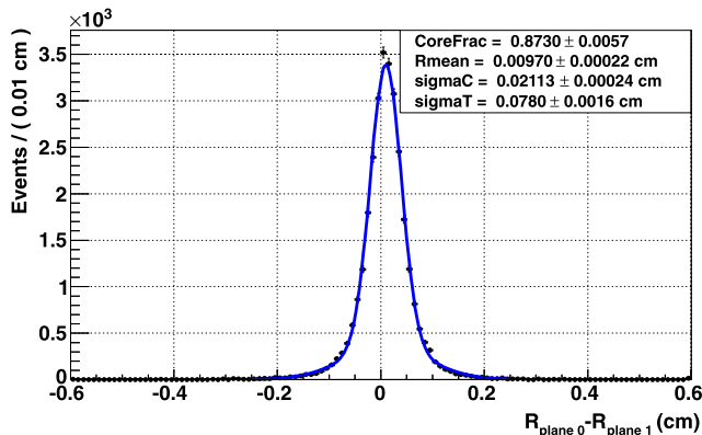
Fig. 29 A fit to the distribution of the difference of projected r coordinates for two-hit clusters
