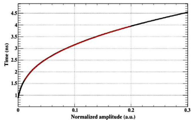
Fig. 42 Time delay versus amplitude relation with fit superimposed
