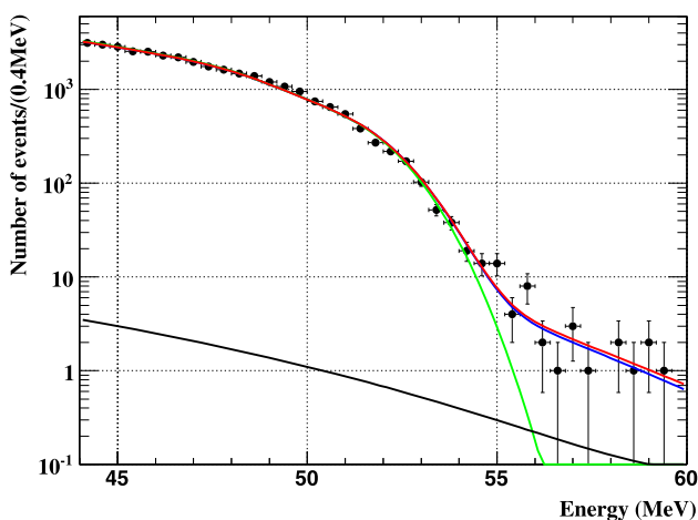
Fig. 59 \gamma -ray background spectrum during physics run in 2010 (see text for details)
