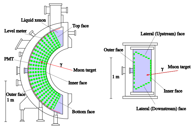
Fig. 48 Schematic view of the LXe detector: from the side ( left ), from the top ( right )
