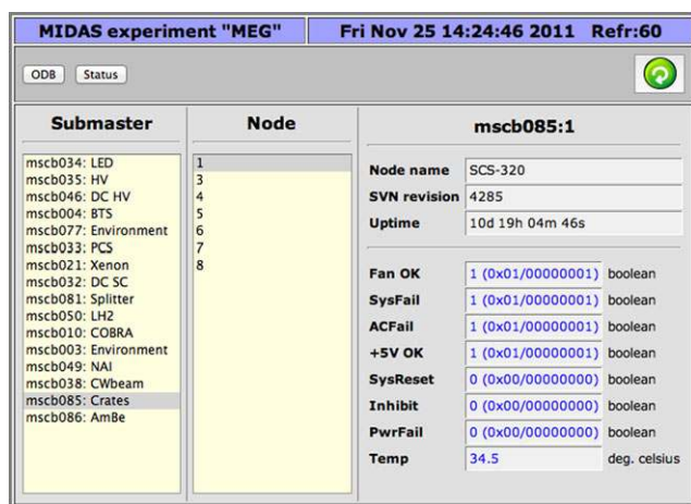
Fig. 84 Web interface page to the MSCB system. The left column shows all available submasters, the second column all nodes connected to the selected submaster, and the right column all network variables of the selected node
