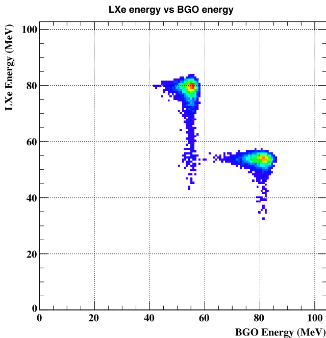
Fig. 72 Energy recorded by the LXe detector vs. the energy recorded by the BGO detector during a CEX calibration run. The extremal energies of the calibration \gamma -rays at 54.9 MeV and 82.9 MeV anti-correlated in the two detectors are visible
