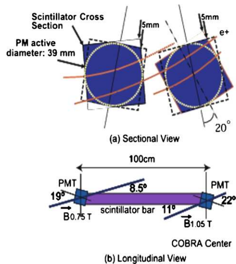
Fig. 37 The layout of a TC bar-PMT assembly
