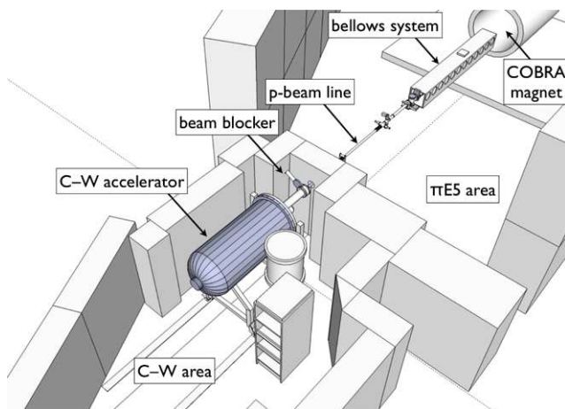
Fig. 67 Schematic layout of the area where the Cockcroft–Walton accelerator is placed, with respect to the \pi E5 area
