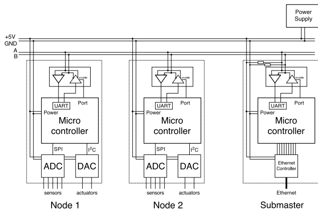
Fig. 82 Simplified communication schematics of the MSCB system
