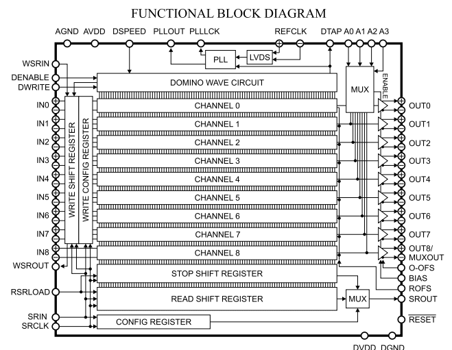
Fig. 79 Functional block diagram of the DRS4 chip
