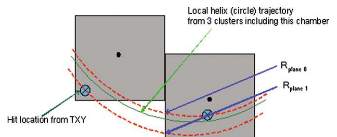
Fig. 28 A diagram of the technique for measuring the intrinsic radial coordinate resolution
