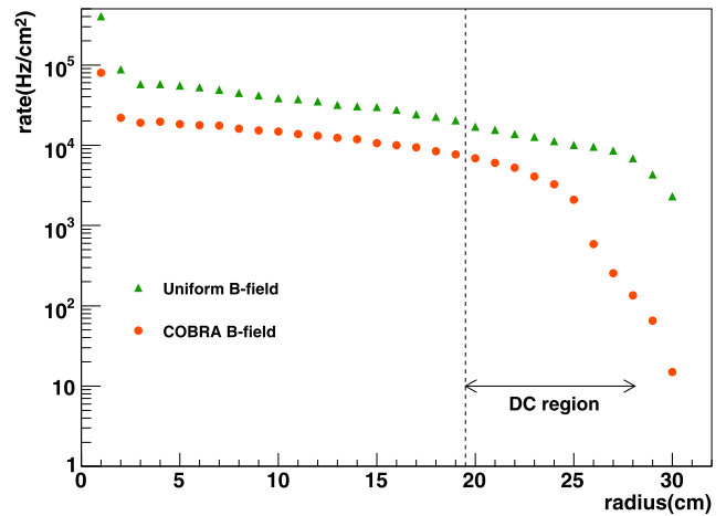
Fig. 14 Hit rate of the Michel positrons as a function of the radial distance from the target in both the gradient and uniform field cases
