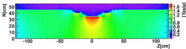
Fig. 16 Gradient magnetic field generated by the COBRA magnet
