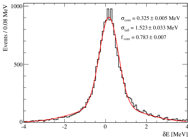
Fig. 35 A fit to the distribution of \delta E_e \equiv E_e^{\text{1st turn}} - E_e^{\text{2nd turn}} on double-turn events. The distribution is fitted with a double Gaussian function convolved with itself, and the corresponding core and tail widths are shown, along with the fraction of events in the core component
