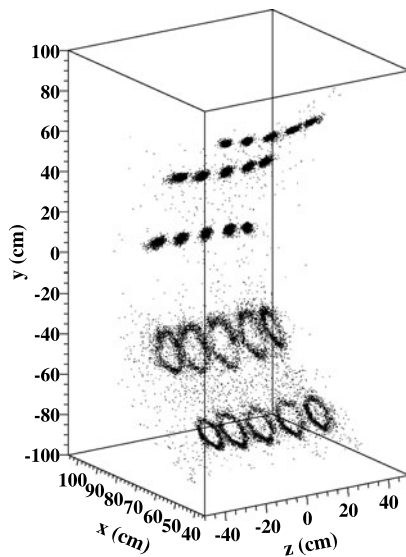
Fig. 60 Reconstructed position of the 25 \alpha -sources inside the LXe detector. In this particular run the detector was partially filled with liquid xenon. The different reconstructed shape of \alpha -sources in gas and in liquid xenon is visible (see text for details)
