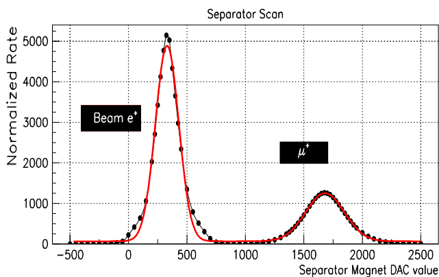
Fig. 3 Separator scan plot, measured post collimator system. The black dots represent on-axis, low discriminator threshold intensity measurements at a given separator magnetic field value during the scan, for a fixed electric field value of -195 kV. The red curve represents a double Gaussian fit to the data points, with a constant background. A separation of 8.1 muon beam \sigma_\mu is found, corresponding to more than 12 cm separation of beam-spot centres at the collimator. The raw muon peak measured at low discriminator threshold also contains a contribution from Michel positrons due to decays in the detector. These can easily be distinguished by also measuring at high threshold, where only muons are visible on account of their higher energy loss and hence higher pulse-height (Color figure online)
