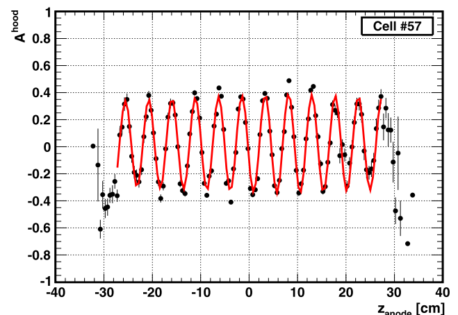
Fig. 26 A fit to the cathode pad asymmetry versus z_{\text{anode}} for the cathode hood of a particular drift cell
