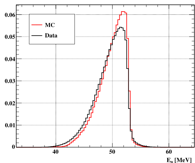
Fig. 88 Normalised momentum spectrum measured in the spectrometer for data and MC simulation
