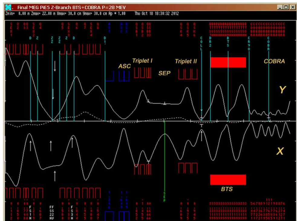
Fig. 5 2nd-order TRANSPORT calculation showing the vertical ( top-half ) and horizontal ( bottom-half ) beam envelopes plotted along the beam-axis from close to target E up to the centre of COBRA, a distance of 22 m. The vertical and horizontal scales differ 33:1. The coloured elements show the vacuum chamber apertures of the various beam elements, while the dotted line represents the central dispersion trajectory for particles with a 1 % higher momentum (Color figure online)
