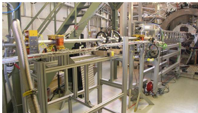
Fig. 68 The Cockcroft–Walton accelerator beam line
