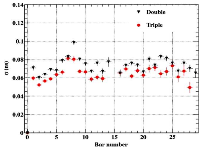
Fig. 46 Timing resolution on double (black markers) and triple (red markers) bar events, with LLT = 25 mV. Due to the different rates for two-bar and three-bar events, the sample used here is different than the one in Fig. 43 (Color figure online)
