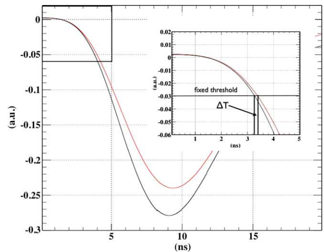
Fig. 41 Graphical representation of the Time Walk effect
