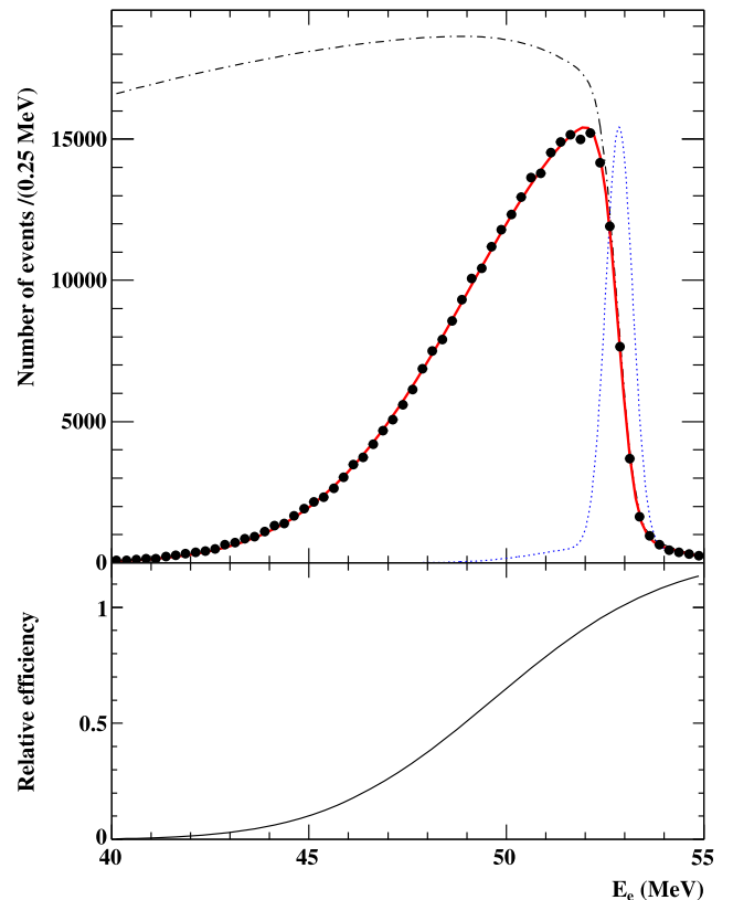
Fig. 34 A fit to the Michel positron energy spectrum. The theoretical spectrum (dashed black), the resolution function (dashed blue) and the acceptance curve (in the bottom plot) are also shown
