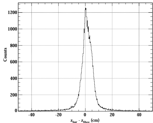
Fig. 39 Distribution of z_{\text{bar}} - z_{\text{fibre}} for the downstream sector
