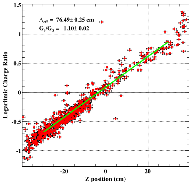
Fig. 47 Logarithm of the PMT charge ratio vs. the z coordinate measured using Eq. (13) for bar number 1. The linear fit returns \Lambda_{eff} and the ratio of PMT gains
