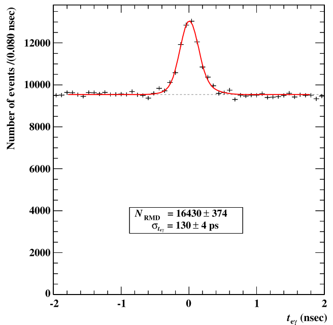
Fig. 73 Distribution of t_{e\gamma} for MEG standard trigger. The peak is from RMDs, the flat component is from accidental coincidences
