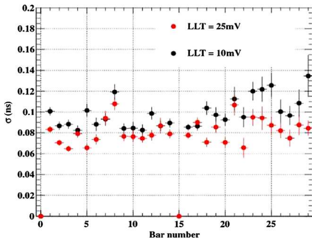
Fig. 43 Timing resolutions for different values of low-level threshold for double bar events
