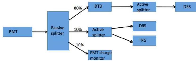
Fig. 38 Schematic picture of the read-out electronics of the TC longitudinal detector. Signals from each PMT are passively split and fed into dedicated electronics channels. Different splitting ratios are used
