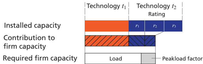
Figure 5: Illustration of system integration constraints with regard to firm capacity: the capacity required to be “firm” (Johnson et al., 2016; Sullivan et al., 2013) depends on yearly average load and a peak-load mark-up; technology t_1 is dispatchable and all installed capacity counts towards firm capacity; technology t_2 depends on variable renewable energy source and different “ratings” counts towards firm capacity at a decreasing rate; the size of each rating bin depends on the share of that technology in the supply portfolio.
