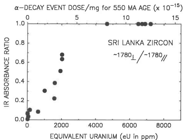
Fig. 6. IR absorbance ratio ( E \perp c ) / ( E // c ) at \sim 1780 \text{ cm}^{-1} as a function of eU and \alpha -decay event dosage. The ratio increases with U content up to approximately 2500 ppm eU, beyond which value the samples are no longer anisotropic.
