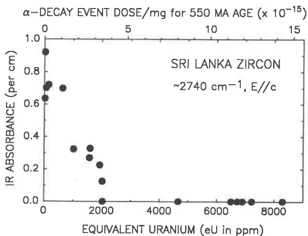
Fig. 8. IR absorbance for polarized single crystal spectra ( E // c ), given in units of absorbance per cm at \sim 2740 \text{ cm}^{-1} , as a function of eU and \alpha -decay event dosage. Band intensity decreases with increasing U content up to about 2500 ppm eU and is negligible above that value.
