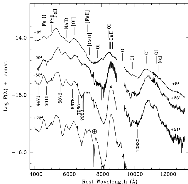
FIG. 9.—Optical and IR spectra of SN 1998bw at comparable phases. Line identifications from spectral modeling are plotted for the most prominent emission features ( top ) and for the He I lines ( bottom ). The He marks are placed at the expected absorption positions for an expansion velocity of 18,300\ \text{km s}^{-1} .
