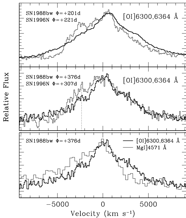
FIG. 12.—Upper and middle panels: The [O I] \lambda\lambda 6300, 6364 line profile at two different epochs for SN 1988bw (thick line) and SN 1996N (thin line; Sollerman et al. 1998). The vertical dotted line is placed at the position of the unidentified feature (see text). Velocities are computed from the \lambda 6300 doublet component. Lower panel: Comparison between the profiles of [O I] \lambda\lambda 6300, 6364 (thick line) and Mg I \lambda 4571 (thin line) for SN 1988bw at +376 days.
