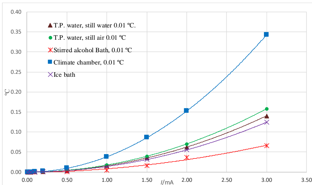
Figure 6. Dependence of the self-heating effect in a PRT with the electrical current applied to the resistance sensing element of the thermometer and dependence of the self-heating effect with the medium surrounding the thermometer
