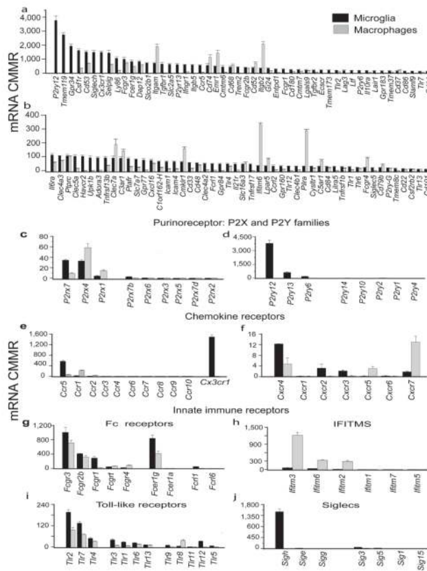
Figure 3. Comparative expression of the microglial and macrophages genes Comparison of expression levels of Sensome genes and those involved in regulating the immune response reveal a distinct immune signature for each cell type. a, b. Expression levels of the microglial Sensome in microglia and macrophages show that several genes are differentially expressed. c. Purinergic P2rx receptors. d. Purinergic P2ry receptors. e. Chemokine Ccr and Cx3cr1 receptors. f. Chemokine Cxc receptors. g. Fc receptors. h. Interferon-inducible transmembrane (Ifitms). i. Toll-like receptors (Tlrs) 1–13. j. Sialic acid binding immunoglobulin lectins (Siglecs). (Values are mean \pm SD of three different experiments done with microglia pooled from 22, 10 and 20 mice, respectively and three pools of macrophages from 10 mice per pool.) Data for Figure 3a–j can be found in Supplementary Table 2.
