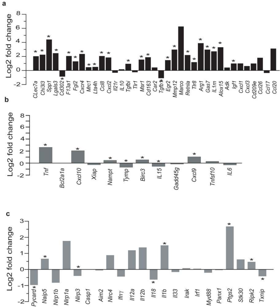
Figure 7. Upregulation of alternative priming genes in microglia from aged mice a,b. Alternative and classical priming genes in microglia from 24 months compared with mice 5 months of age old mice show a wide range of expression levels. a. In old mice, 24 of 37 alternative priming state markers were statistically significantly upregulated (*p<0.016). b. In 24 months old vs. microglia from 5 months old mice, 5 of 12 markers of the classical priming state were significantly upregulated in microglia, while the remaining 7 were down-regulated or not significantly changed. c. Analysis of 22 inflammasome-associated genes shows that 4 are significantly up-regulated in old mice compared with young ones (*p<0.025), while the remaining 18 genes are down-regulated or not significantly changed. Taken together the data suggest a trend toward increased expression of genes involved in resolution of inflammation and neuroprotection. Values are Log2 Fold change of three
