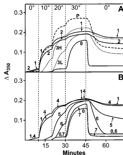
FIGURE 2: Drug-induced tubulin assembly in the presence of MAPs and GTP. Reaction mixtures (final volume, 0.25 mL) containing all components except the drug were placed in cuvettes held at 0 ^\circ\text{C} in Gilford model 250 spectrophotometers equipped with electronic temperature controllers. Baselines were established at 350 nm, and the drug was added in dimethyl sulfoxide (final concentration, 1%). Turbidity changes were followed, with the indicated temperature changes made at the time points indicated by the dashed lines to the left of the temperature. Reaction mixtures contained 0.1 M 4-morpholineethanesulfonate (pH 6.9 with NaOH in 1 M stock solution), 10 \mu\text{M} (1.0 mg/mL) tubulin, 0.75 mg/mL heat-treated MAPs, and 0.1 mM GTP. (A) Curve 0, no drug; P, 10 \mu\text{M} paclitaxel; 1, 10 \mu\text{M} laulimalide; 2, 10 \mu\text{M} epothilone A; 3L, 10 \mu\text{M} trans -desoxyaulimalide; 3H, 40 \mu\text{M} trans -desoxyaulimalide. (B) Curve 0, no drug; 1, 10 \mu\text{M} laulimalide; 4, 10 \mu\text{M} eleutherobin; 5, 10 \mu\text{M} sarcodictyin A; 6, 10 \mu\text{M} 2-ethoxyestradiol analogue; 7, 10 \mu\text{M} baccatin III.
