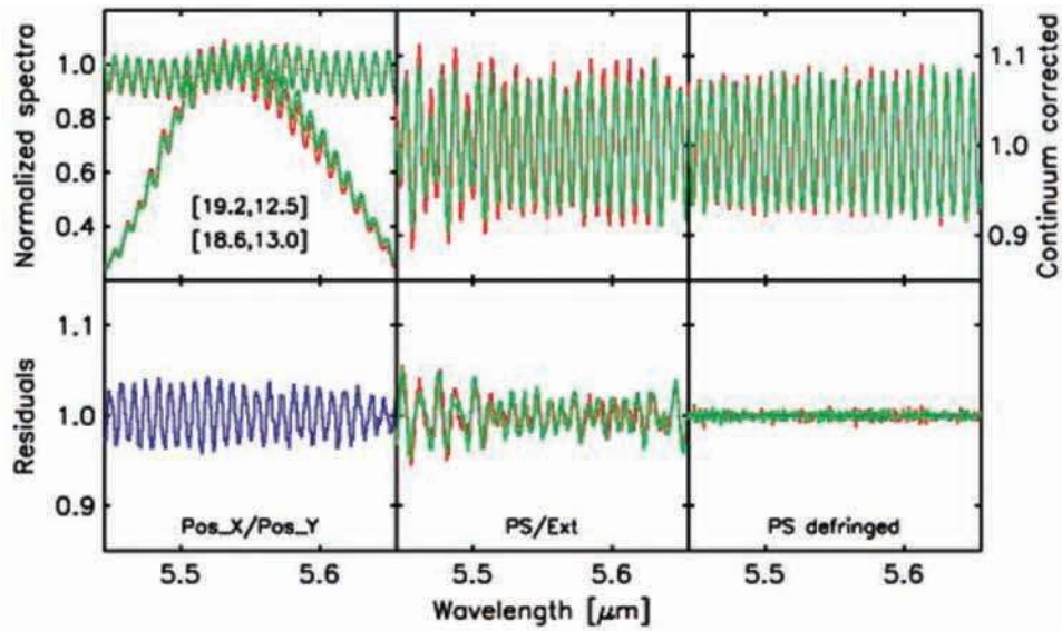
Fig. 19.— Illustration of the fringe source dependence for point and extended blackbody source spectra at two positions (red and green spectra) as printed in the top-left panel. Top from left to right; peak normalized point and extended spectra; normalized point source spectra; normalized extended blackbody spectra. Bottom from left to right; both point source spectra divided; point source spectra divided by extended source spectra (akin to direct flat-field correction); both normalized point source spectra de-fringed using a sine fitting technique.
