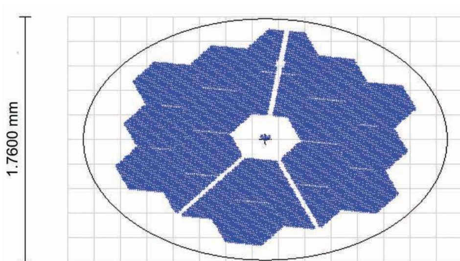
Fig. 5.— Rotated and anamorphically magnified pupil image at the entrance to the IFU of Channel 3, plotted on a square grid.
