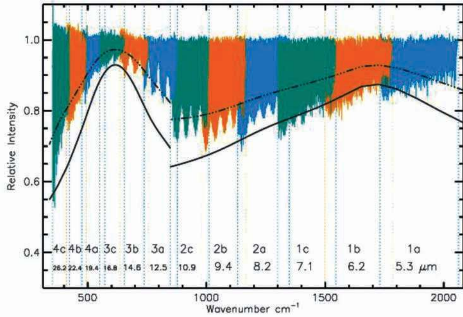
Fig. 18.— The combined fringes for each channel and sub-band. The data for each neighbouring band are plotted in a different colour for clarity. The main and high frequency fringe components are not resolved on this scale. In Channels 2 and 3 an example of a low frequency beating fringe can clearly be seen. Note: the spectrum is normalized to the peaks of the main fringe amplitude. See text for a description of the solid and dashed-dotted lines.
