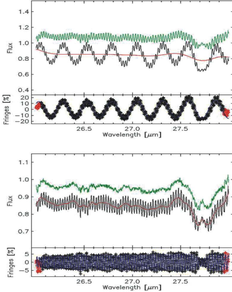
Fig. 17.— Examples of two main observed MRS fringe components. In the top panels of each plot the input data is shown in black with a fitted continuum in red. The spectrum (offset for clarity) after fringe removal is shown in green. In the lower panels the normalized spectrum and fitted fringes are shown. Top: the main component #1 in Channel 4 (after de-fringing, fringe component #2 remains); bottom: the high frequency fringe component #2.
