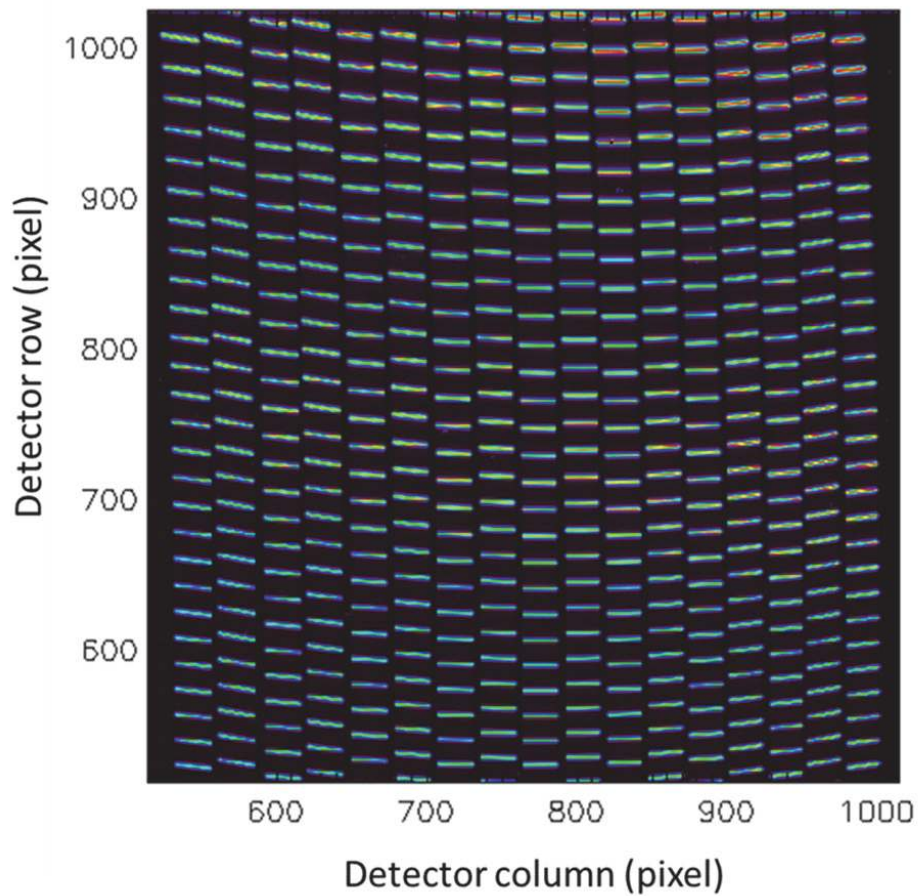
Fig. 13.— A typical wavelength calibration observation. The long wavelength half of Sub-band 2A is shown when illuminated by an extended continuum source modulated by a vacuum spaced etalon with a free spectral range (fringe spacing) of 3.1 \text{ cm}^{-1} at ambient.
