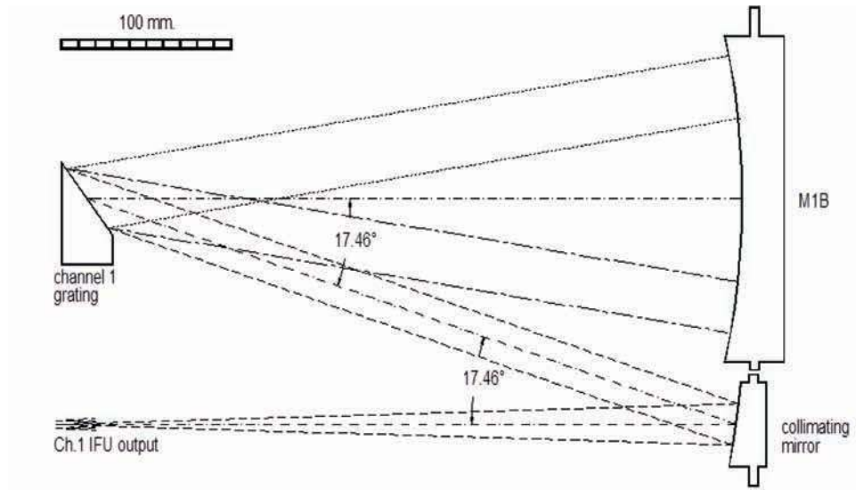
Fig. 9.— Cross-section along the dispersion direction of the collimator, grating and camera mirror M1 of the SMO.
