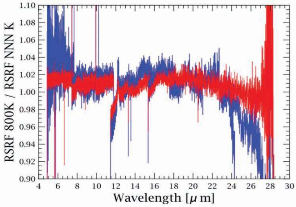
Fig. 21.— Comparison of the Relative Spectral Response function calculated using observations of the MTS black body at 400 K (blue) and at 600 K (red) with the RSRF at 800 K.
