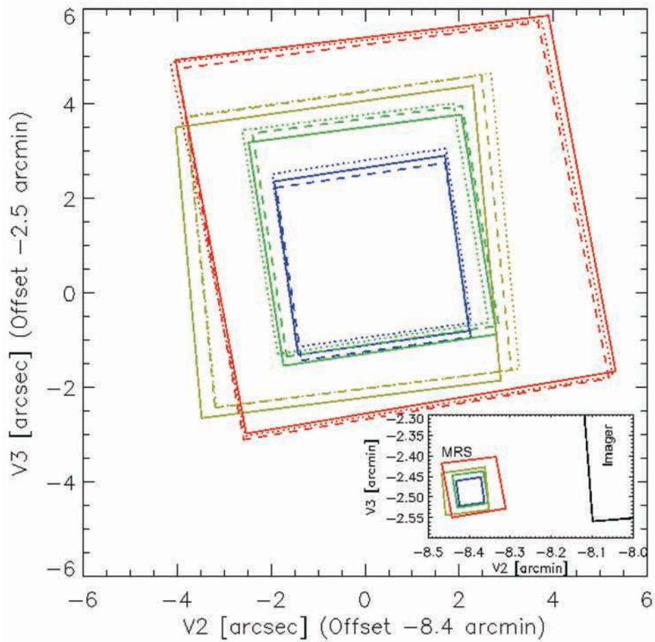
Fig. 12.— Transformed MRS fields in the JWST coordinate frame ( V_2 , V_3 ). The field borders are drawn as solid lines (Sub-band A), dashes (Sub-band B) and dots (Sub-band C) for channel 1 (blue), 2 (green), 3 (yellow) and 4 (red). The inset shows the position of the MRS FOV relative to the imager field.
