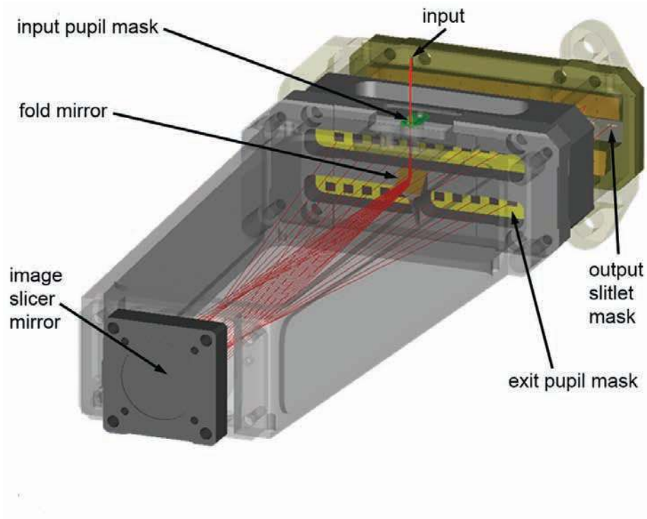
Fig. 4.— Three Dimensional View of the Channel 3 IFU.
