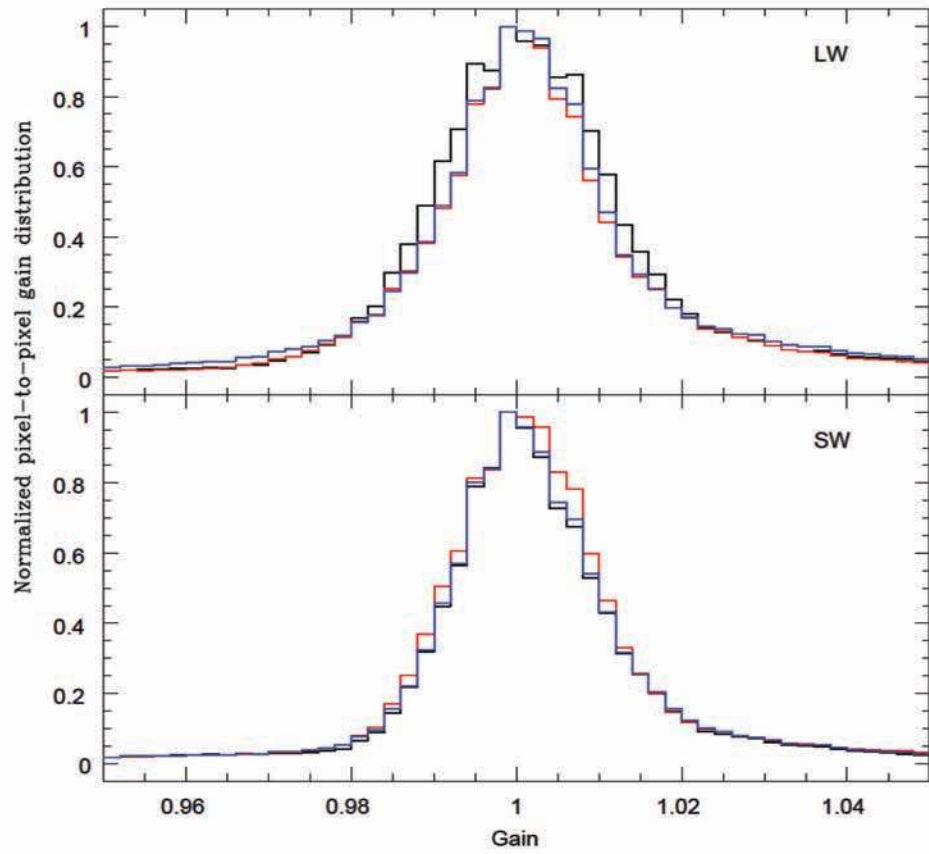
Fig. 20.— Normalized pixel-to-pixel gain distributions derived from 3 observations for SW and LW detectors (black, red and blue). The FWHMs are 1.91 % and 1.99 % for the SW and LW channels, respectively.
