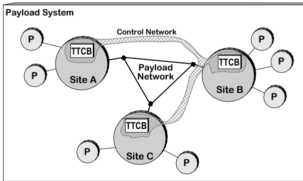
Figure 2. Trusted Timely Computing Base Model
