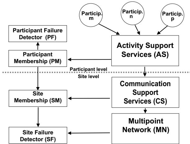
Figure 4. Architecture of a MAFTIA Node
