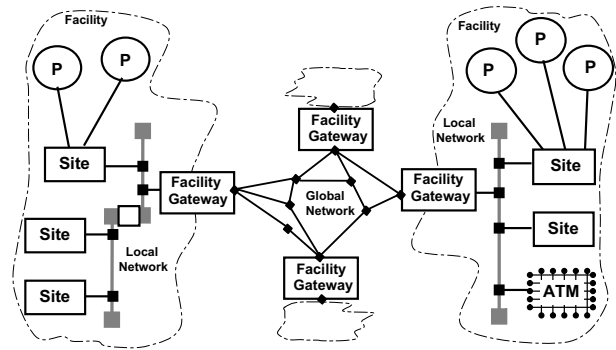
Figure 3. Two-tier WAN-of-LANs
