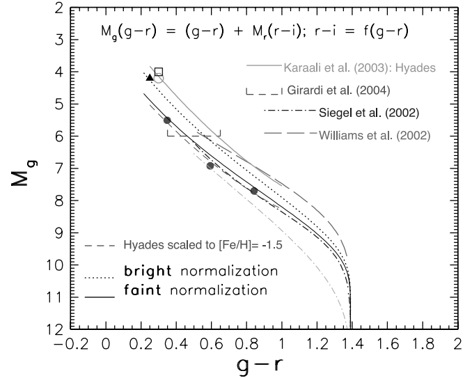
FIG. 3.—Comparison of photometric parallax relations from the literature and adopted in this work, shown using SDSS bands (stars with spectral types later than \sim M0 have g - r \sim 1.4 ). The two relations adopted here are shown by the dotted (“bright” normalization) and solid (“faint” normalization) lines. These are the same relations as shown in Fig. 2, translated here into the M_g(g - r) form using the r - i = f(g - r) relation appropriate for MS stars on the main stellar locus. Other lines show photometric parallax relations from the literature, as marked. The line marked Girardi et al. shows the range of model colors for M_g = 6 . The bottom thin line from Siegel et al. corresponds to low-metallicity stars. The triangle, circle, and square show the SDSS observations of globular cluster Pal 5 ( [Fe/H] = -1.4 ) and the Hyades ( [Fe/H] = 0.1 ) and M48 ( [Fe/H] = -0.2 ) open clusters, respectively. The three large dots show the SDSS observations of globular cluster M13 ( [Fe/H] = -1.5 ). Note the good agreement between these observations and the Hyades sequence scaled to M13’s metallicity using the prescription from Laird et al. (1988). For reference, B - V = 0.95(g - r) + 0.20 to within 0.05 mag. [See the electronic edition of the Journal for a color version of this figure.]
