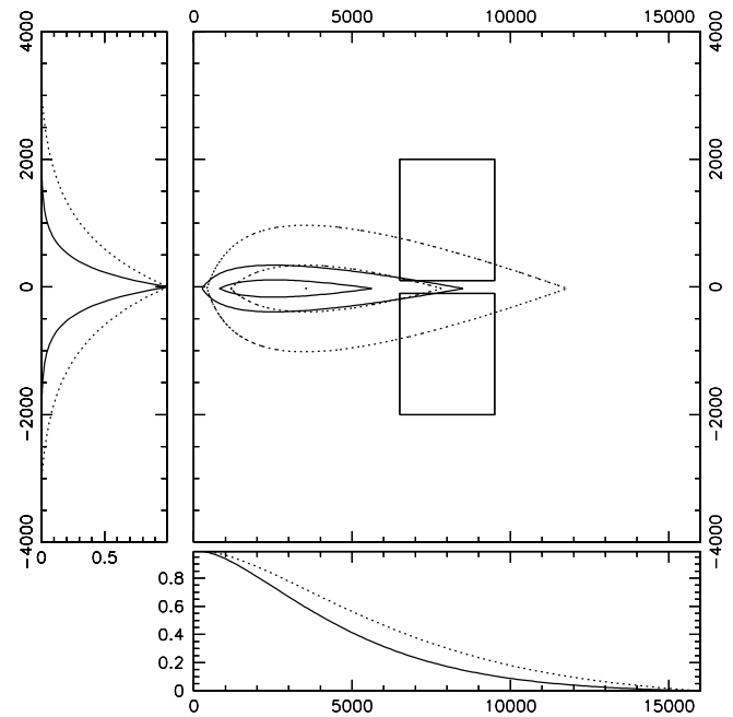
FIG. 41.—Mass contribution to thin (solid lines) and thick (dotted lines) disks from different radii and heights in the Galaxy. Center panel shows the isodensity contours of thin (solid lines) and thick (dotted lines) disks having the bias-corrected parameters of Table 10. Two rectangles centered around R = 8 kpc enclose the range in radii and vertical distances Z from the disk from which the model parameters were measured. The bottom panel shows the cumulative fraction of disk mass enclosed outside a given radius R . Similarly, the left panel shows the fraction of disk mass enclosed at heights |Z| > |Z_{\text{given}}| . Note that while our coverage in the Z -direction is adequate, in the R -direction we sample a region that contains less than 20% of the total disk mass and extrapolate the obtained density laws toward the Galactic center where most of the mass lies.
