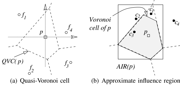
Fig. 4. Examples of the QVC method
