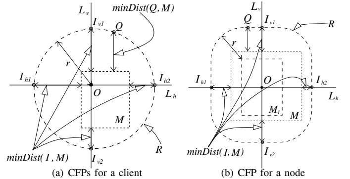
Fig. 7. Candidate furthest points
