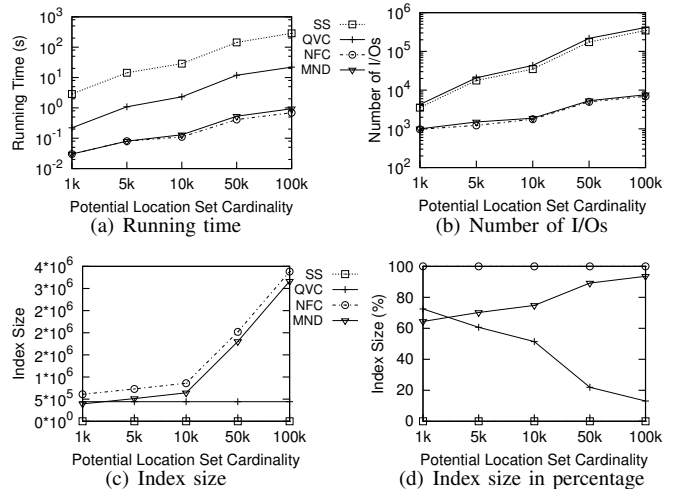
Fig. 12. The effect of potential location set size
